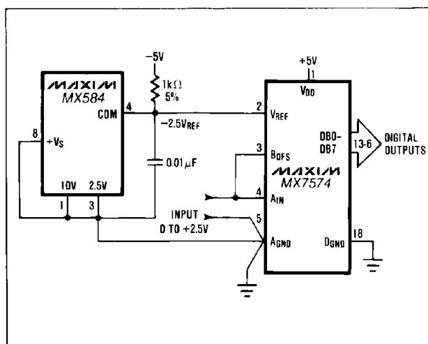
Figure 11. MX584 as Negative 2.5 Volt Reference for a CMOS ADC
