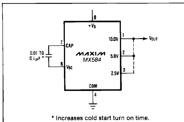
Figure 4. Additional Noise Filtering with an External Capacitor
