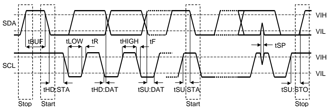
Figure 2. I²C Bus Mode Timing
