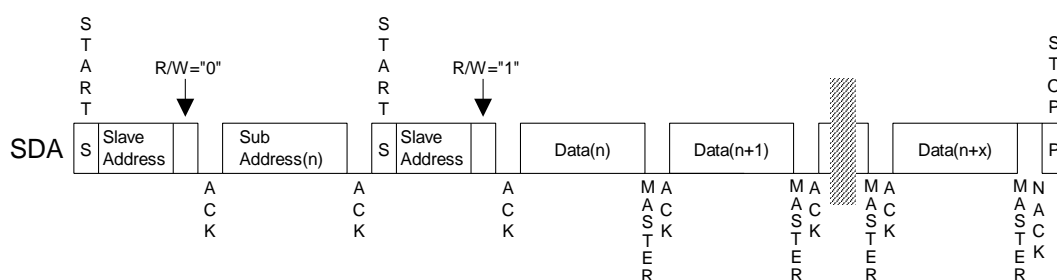
Figure 13. Random Address Read
