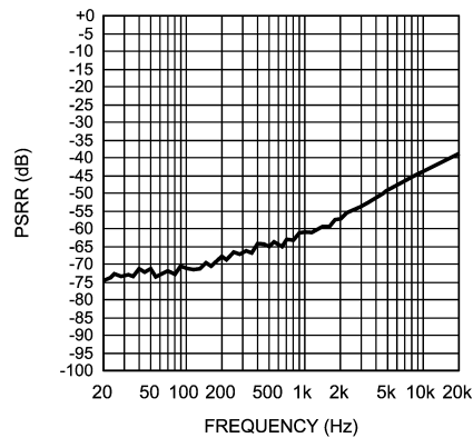
PSRR vs Frequency V_1 = 5.0V , Z_L = 2\mu F + 30\Omega , V_{ripple} = 200mV_{pp} , A_{V-BTL} = 26dB
