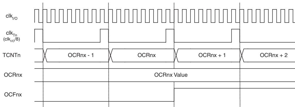
Figure 15-10. Timer/Counter Timing Diagram, Setting of OCF0A, with Prescaler ( f_{\text{clk\_I/O}}/8 )
