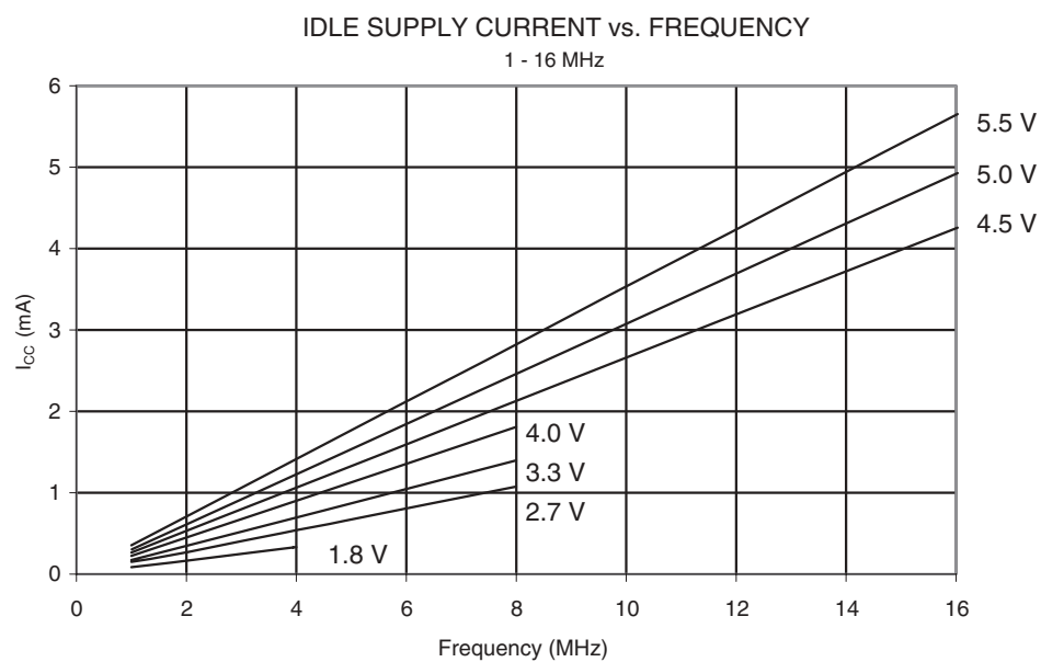
Figure 29-7. Idle Supply Current vs. Frequency (1 - 16 MHz)
