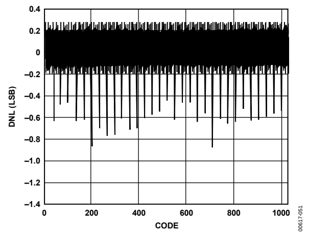
Figure 51. Typical DNL
