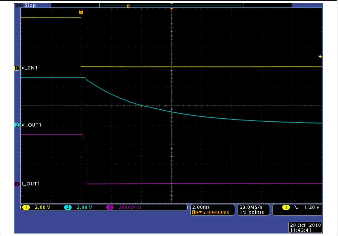
Figure 14. Turn-off for C LOAD = 470 μF
