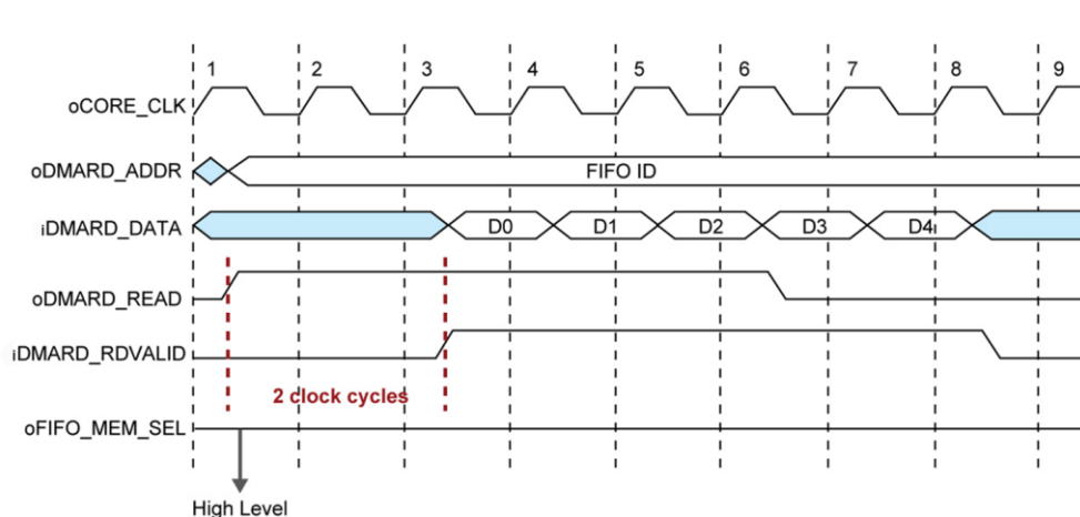
Figure 6-5 Write Transaction Waveform of the PCIe DMA channel on memory mapping mode
