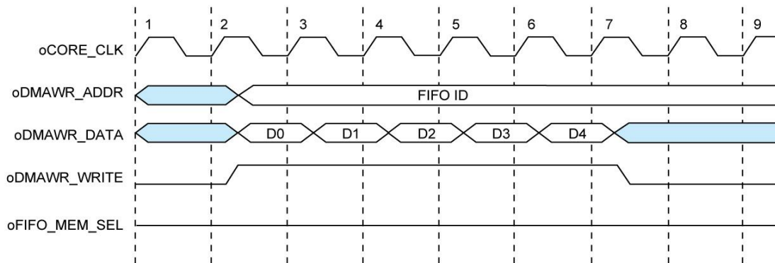
Figure 6-7 Write Transaction Waveform of the PCIe DMA Channel in FIFO-link Mode
