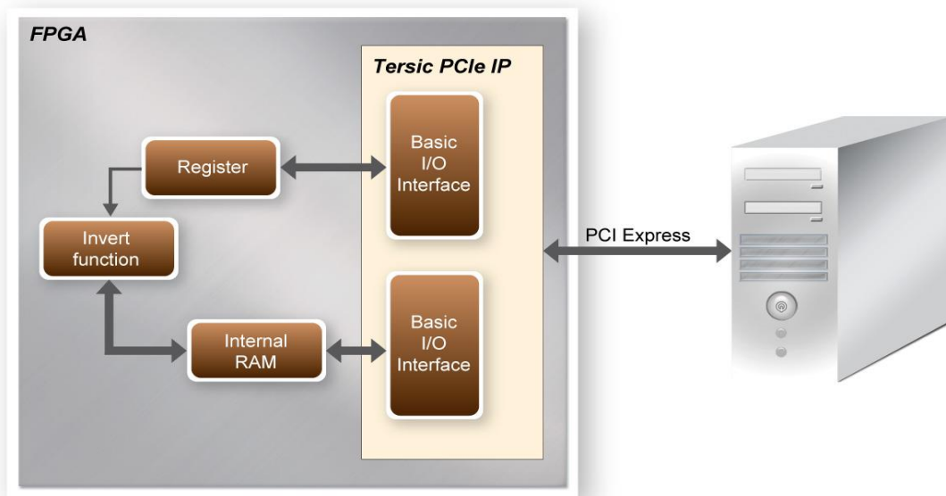
Figure 6-15 Block Diagram of Image Processing Reference Design
