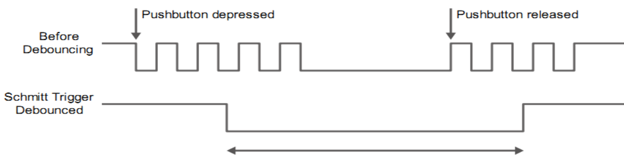
Figure 2-10 Push-button Debouncing
