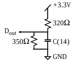
Figure C: Output load
