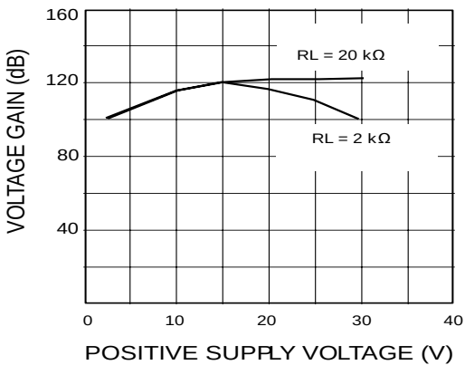
Figure 12: Open-loop gain
