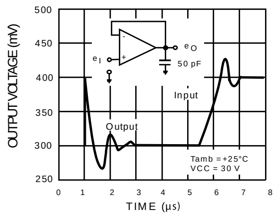
Figure 6: Voltage follower pulse response with VCC = 30 V
