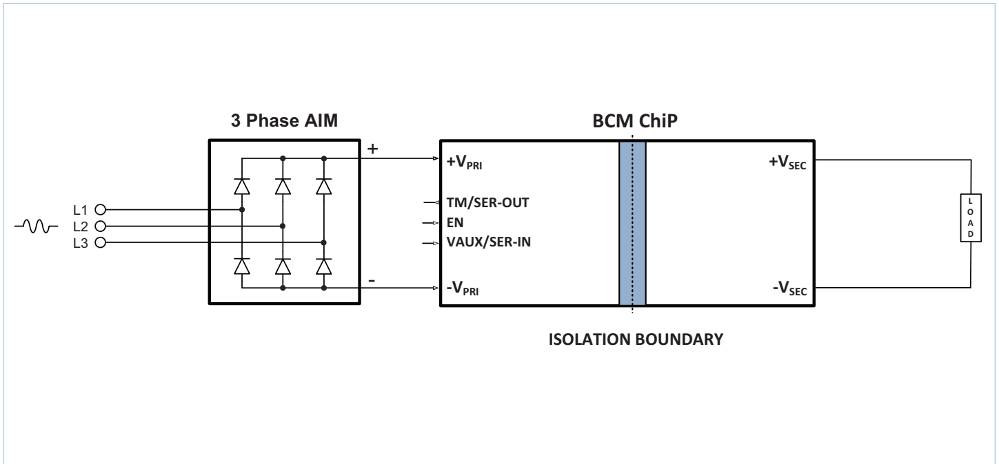
3 phase AC to point of load (3 phase AIM + BCM6123xD0G5030yzz)
