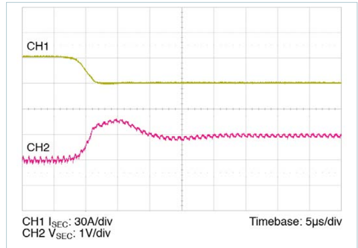
Figure 16 — 30A – 0A transient response: C_{PRI\_IN\_EXT} = 10\mu F , no external C_{SEC\_OUT\_EXT}
