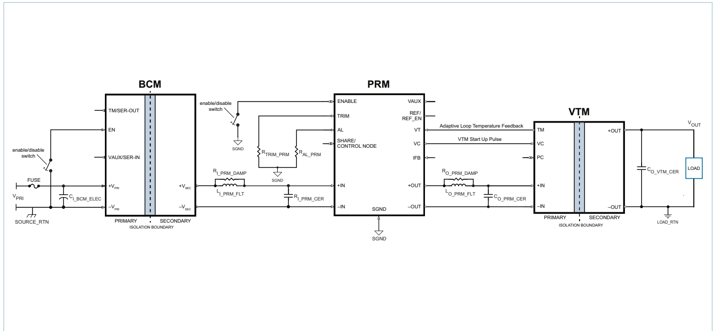
BCM6123xD0G5030yzz + PRM + VTM, Adaptive Loop Configuration
