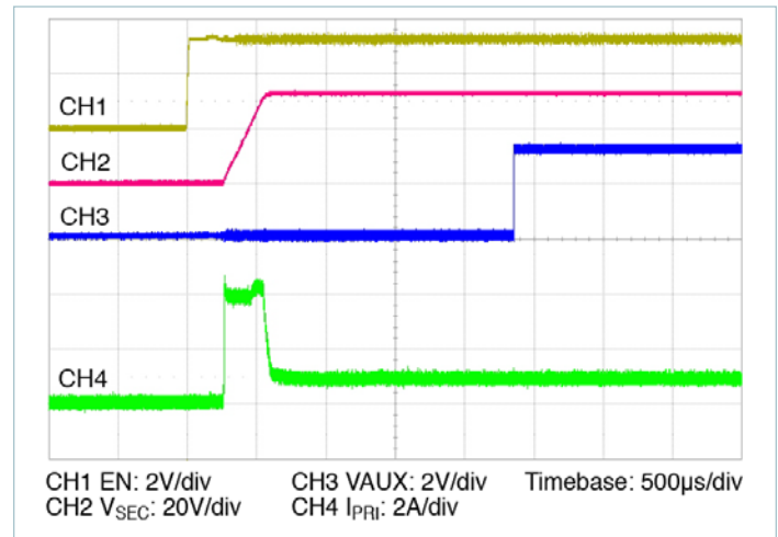
Figure 18 — Startup from application of EN with pre-applied V_{PRI\_DC} = 270V , 20% I_{SEC\_OUT\_DG} , 100% C_{SEC\_OUT\_EXT}
