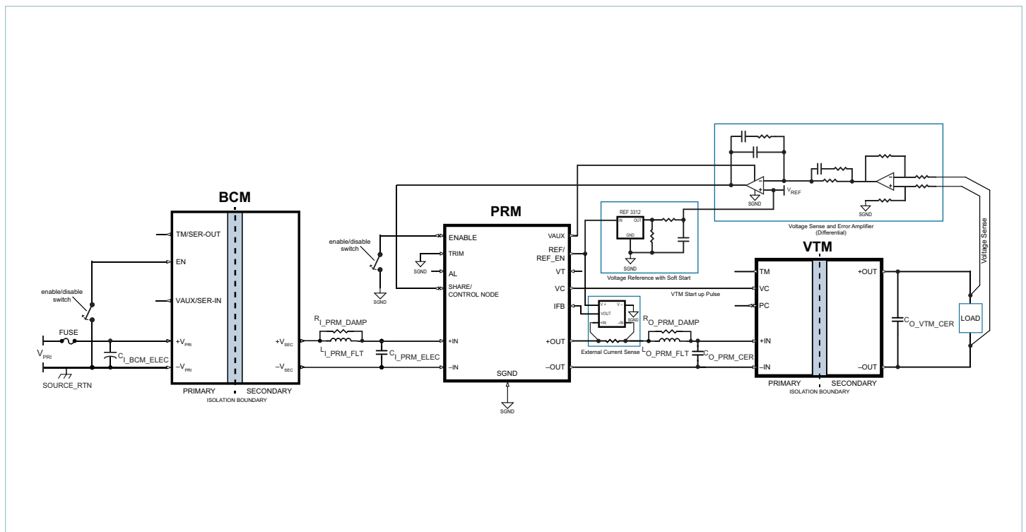
BCM6123xD0G5030yzz + PRM + VTM, Remote Sense Configuration
