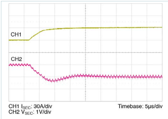
Figure 15 — 0A – 30A transient response: C_{PRI\_IN\_EXT} = 10\mu F , no external C_{SEC\_OUT\_EXT}
