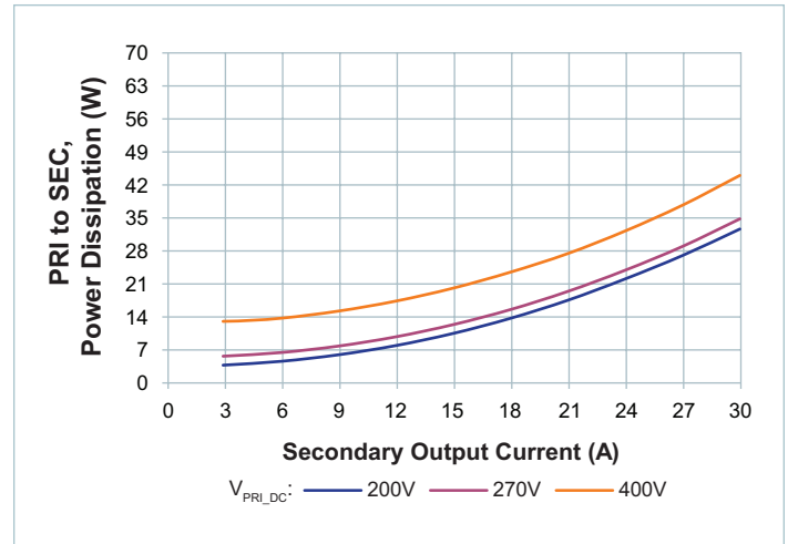
Figure 11 — Power dissipation at T_{CASE} = 100^{\circ}\text{C}
