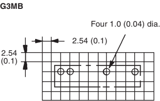
PCB Dimensions (Bottom view)
