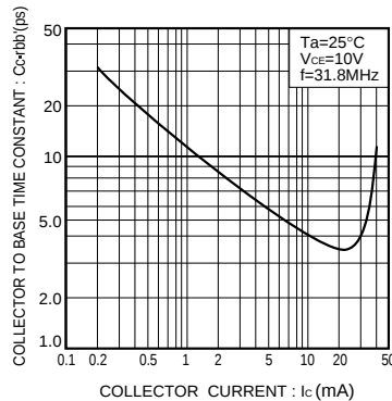
Fig.5 Collector to base time constant vs. collector current characteristics
