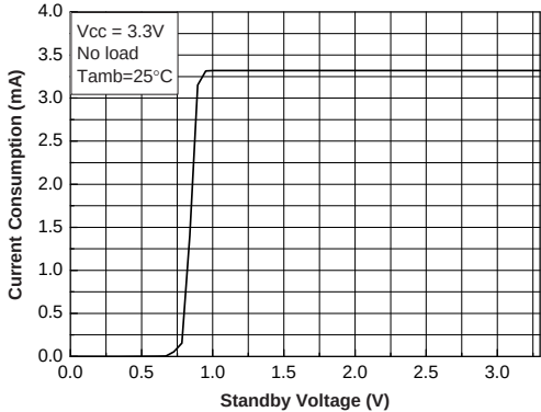
Figure 41. Current consumption vs. standby voltage @ V_{CC} = 3.3\text{ V}
