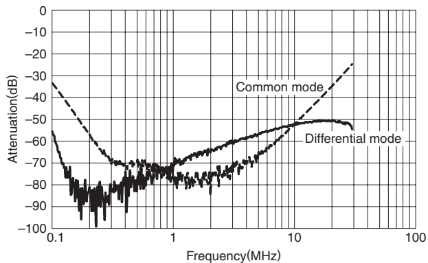
RTHC-5040
