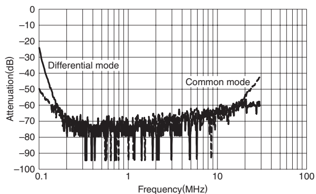
RTHC-5010
