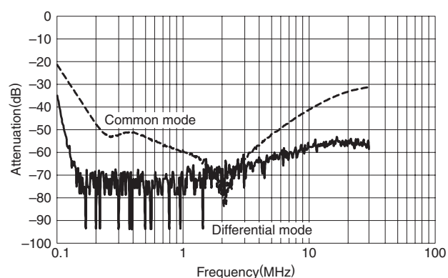
RTHC-5200
