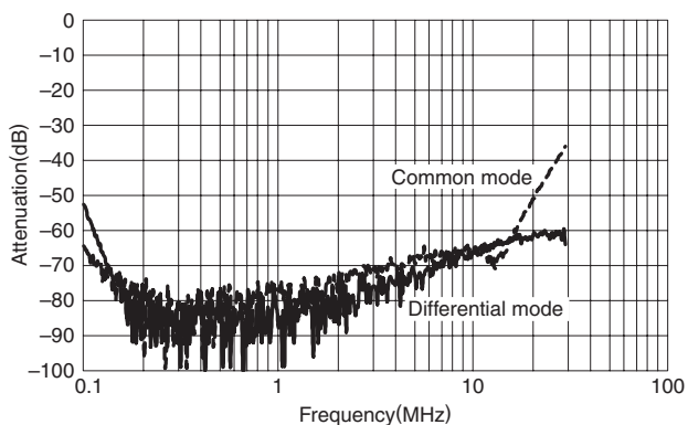
RTHC-5006
