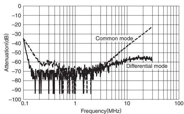
RTHC-5150
