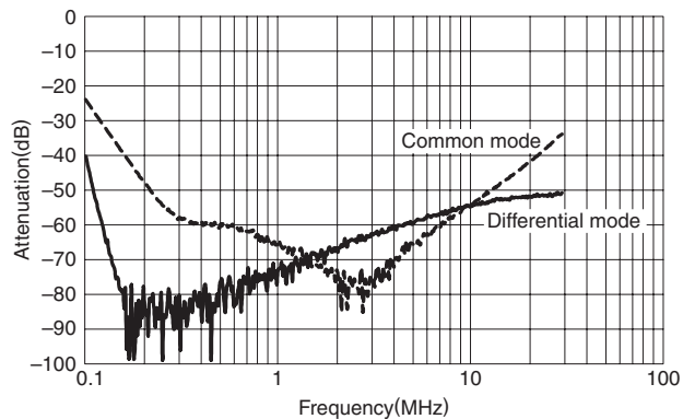
RTHC-5050
