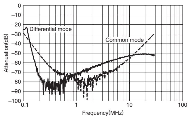
RTHC-5030
