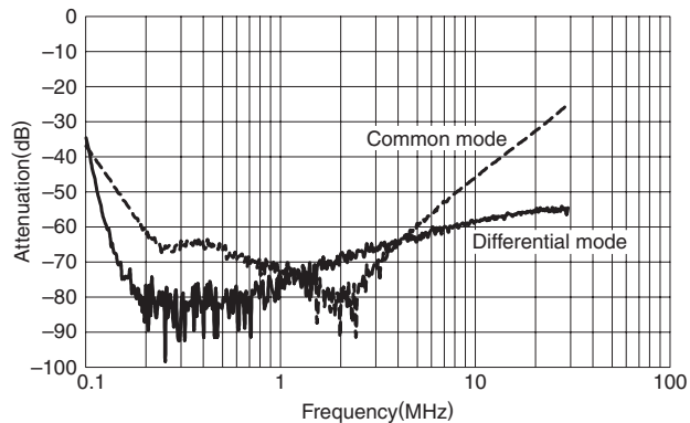
RTHC-5080
