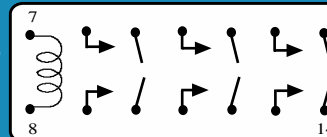
219FXXP 6P-NO
