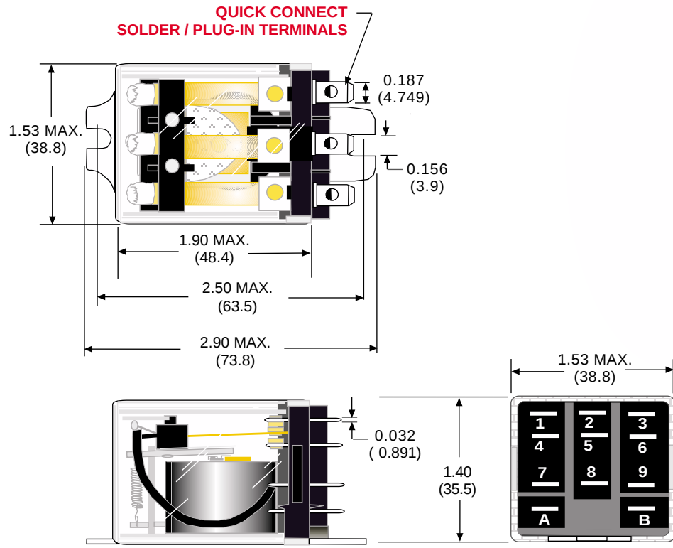
OUTLINE DIMENSIONS DIMENSIONS SHOWN IN INCHES & (MILLIMETERS).
