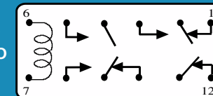
219ABAP DPDT+1NO & 1NC
