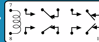
219DXDP 4PDT
