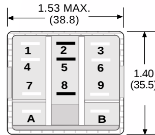
OUTLINE DIMENSIONS DIMENSIONS SHOWN IN INCHES & (MILLIMETERS).
