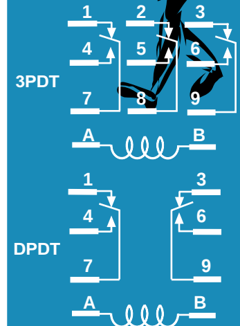
WIRING DIAGRAMS (VIEWED FROM PIN END)
