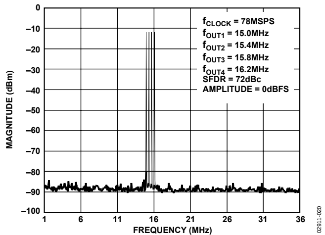
Figure 21. Four-Tone SFDR
