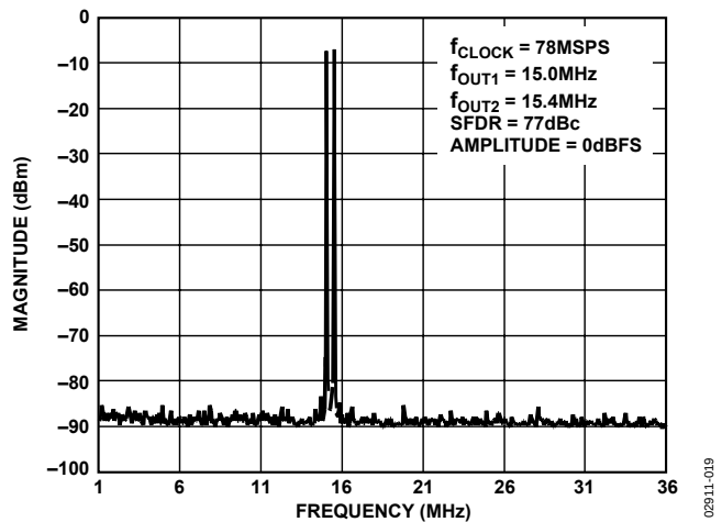
Figure 20. Dual-Tone SFDR
