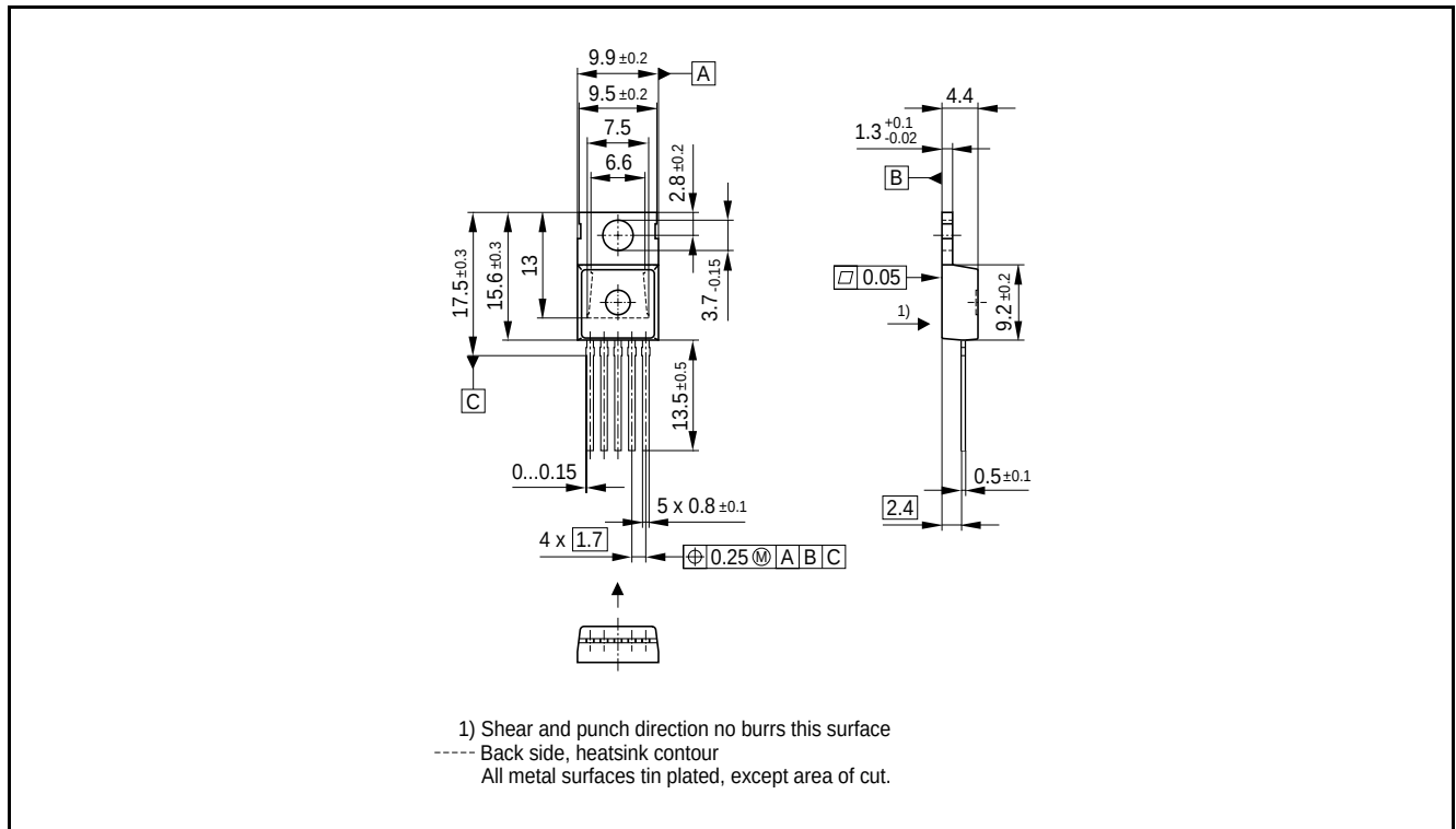
Figure 3 PG-T0220-5-43
