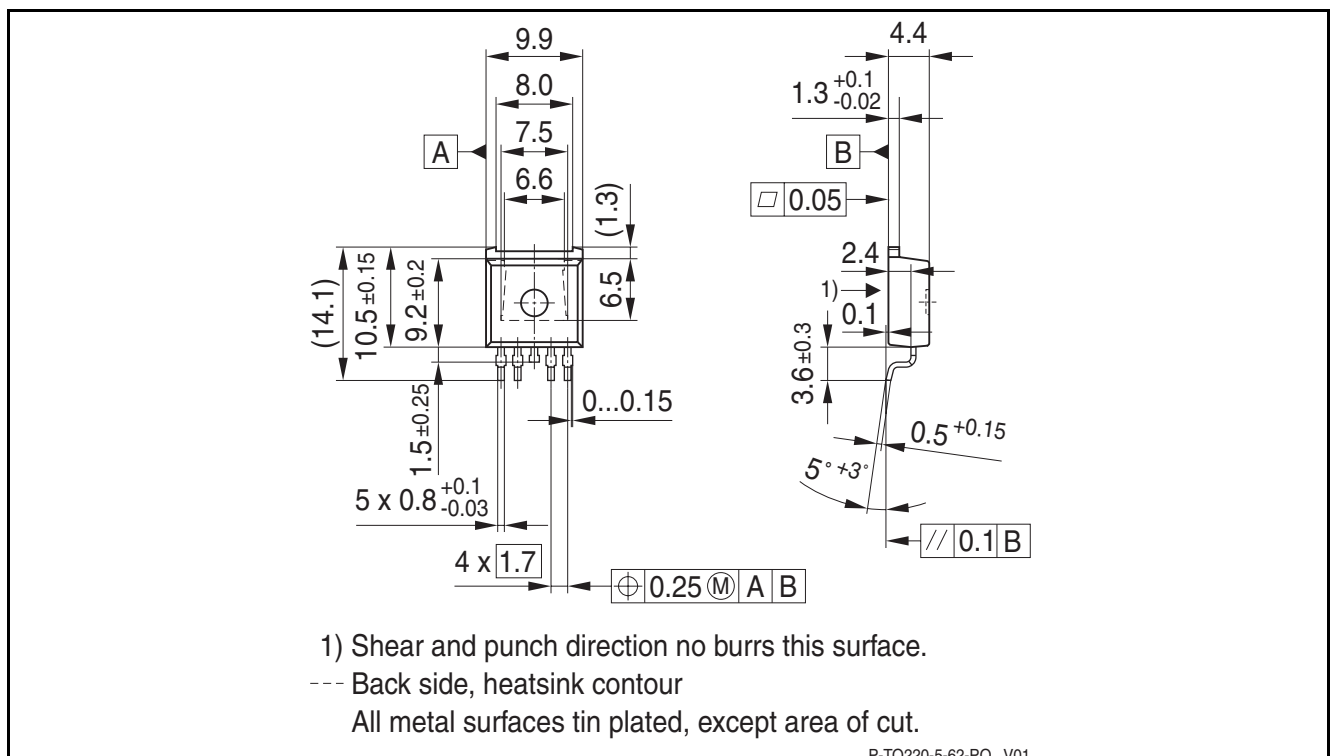
Figure 2 PG-TO220-5-62
