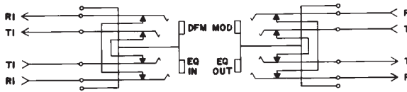
TYPICAL CIRCUIT ARRANGEMENT
