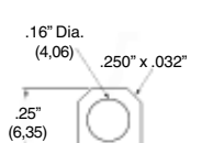
S 2 Solder Eye, extra large & quick connect
