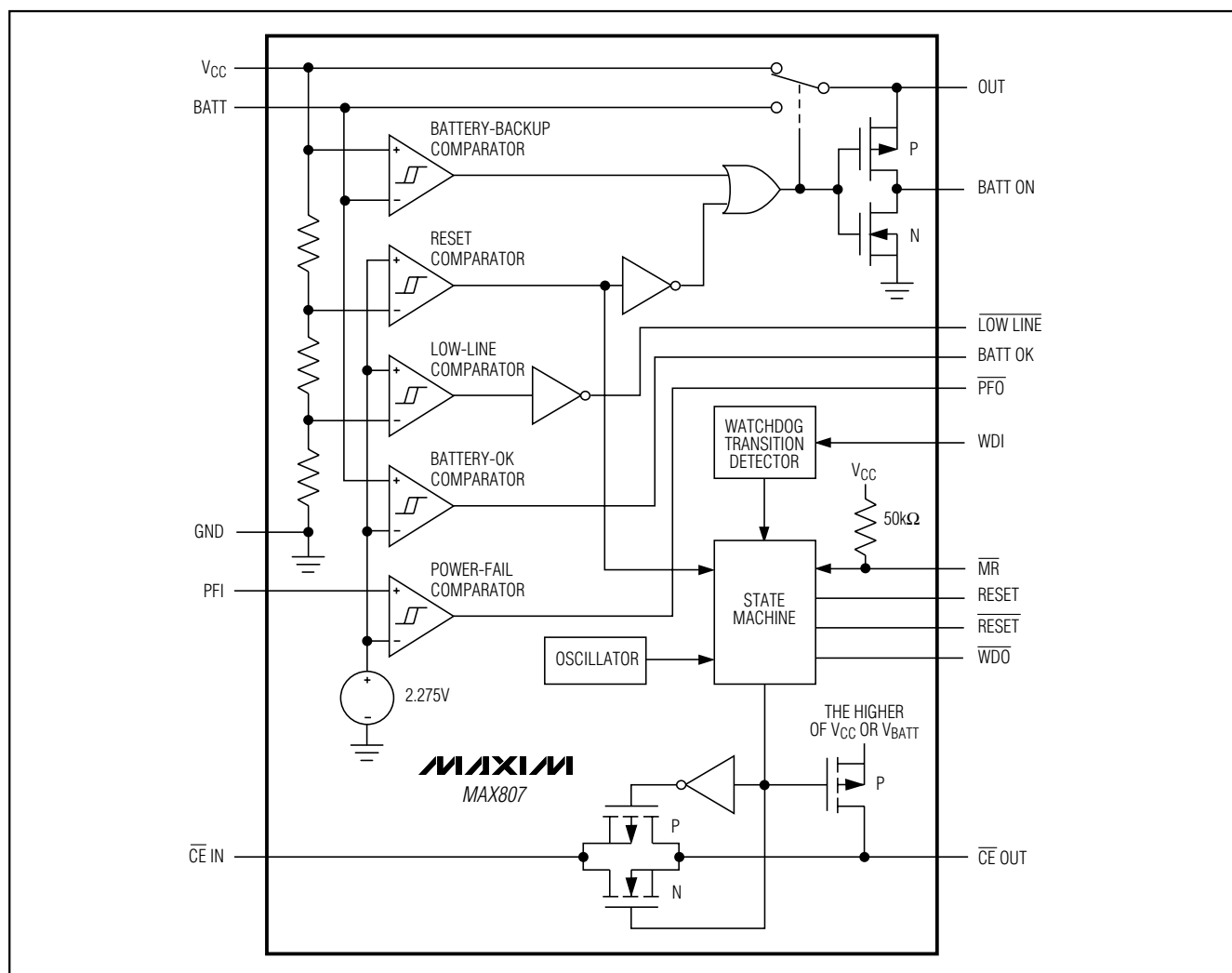
Figure 1. Block Diagram
