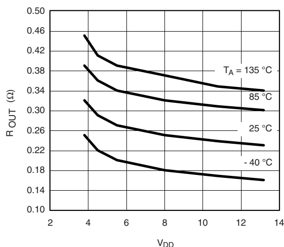
R_{OUT} vs. V_{DD}
