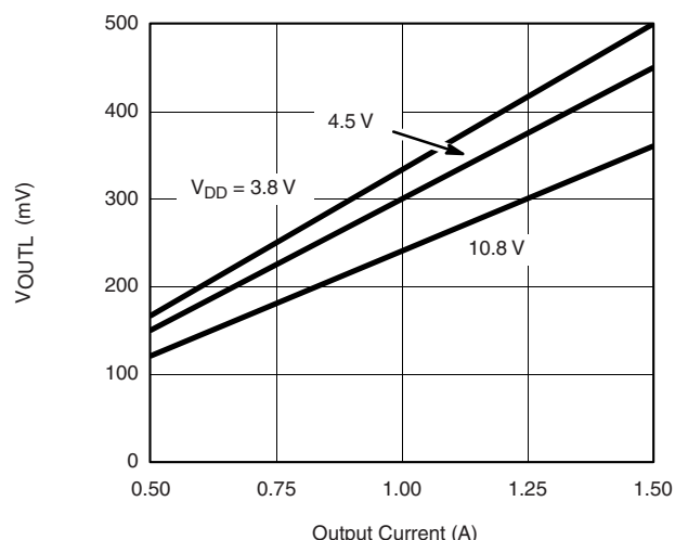
Output Low Voltage vs. Output Current
