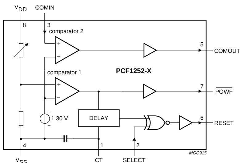
Fig.1 Block diagram.
