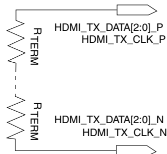
Figure 58. Source Termination
