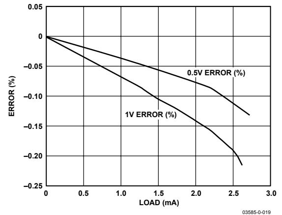
Figure 34. VREF Accuracy vs. Load
