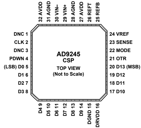
Figure 3. 32-Lead LFCSP
