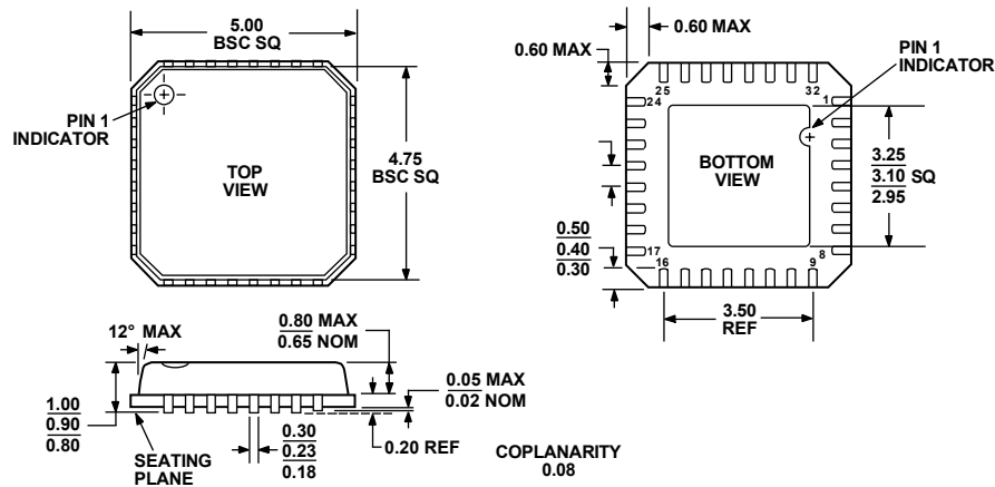
Figure 46. 32-Lead Frame Chip Scale Package [LFCSP] (CP-32) Dimensions shown in millimeters
