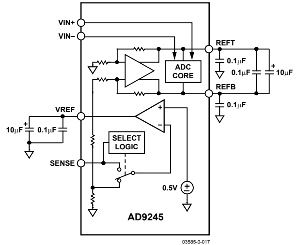
Figure 33. Internal Reference Configuration
