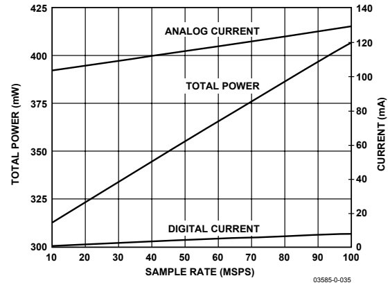
Figure 32. Power and Current vs. Sample Rate @ 2.5 MHz
