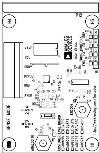
Figure 44. LFCSP Evaluation Board Layout, Primary Silkscreen
