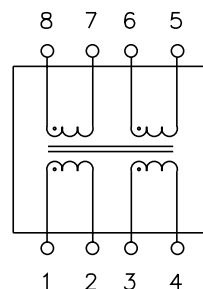
Circuit Diagram B
