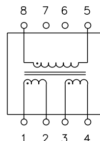
Circuit Diagram A
