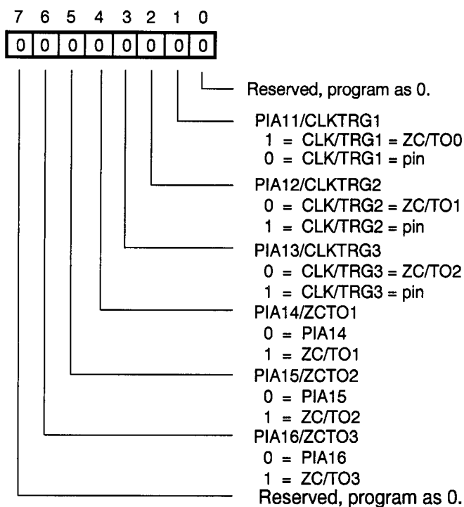
PIA1/CTC Pin Select Register (I/O Address %DE)
