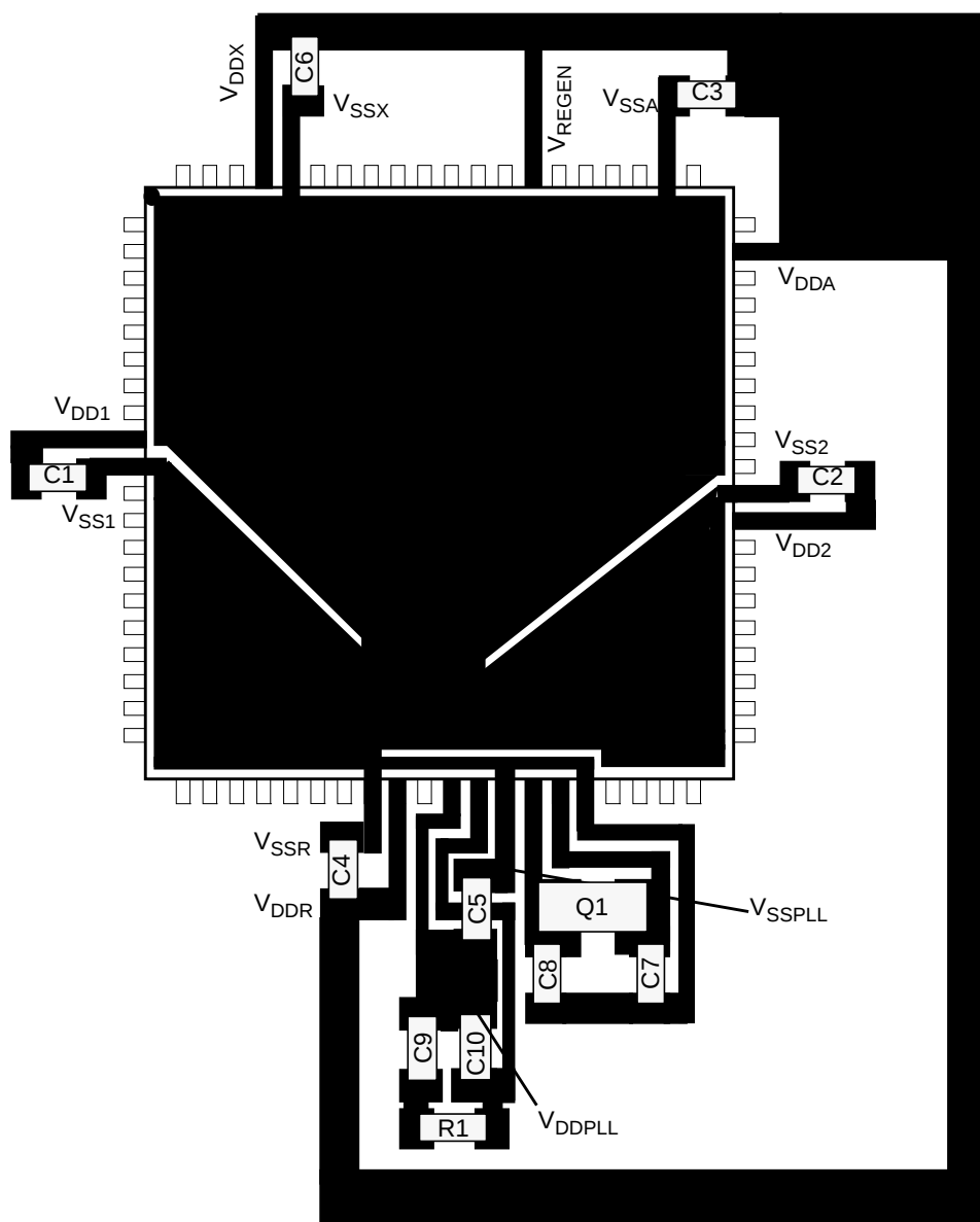
Figure C-3. 80-Pin QFP Recommended PCB Layout
