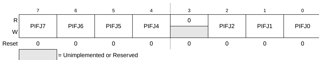
Figure 22-63. Port J Interrupt Flag Register (PIFJ)
