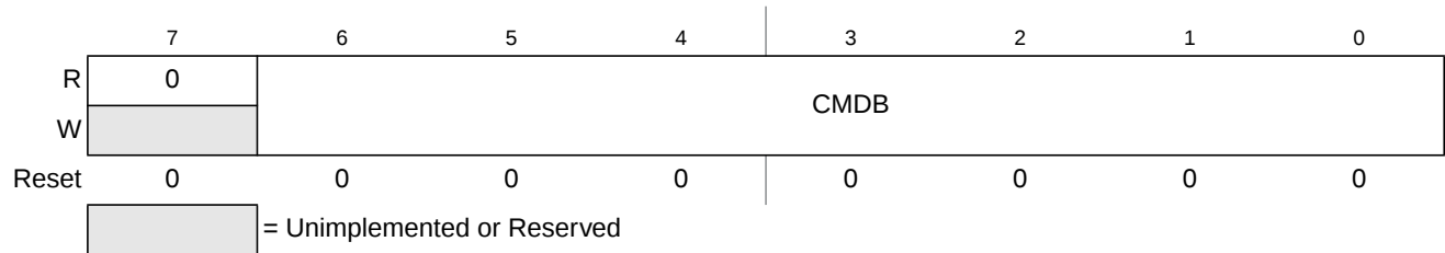
Figure 26-11. EEPROM Command Register (ECMD)
