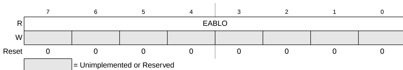
Figure 25-14. EEPROM Address Low Register (EADDRLO)
