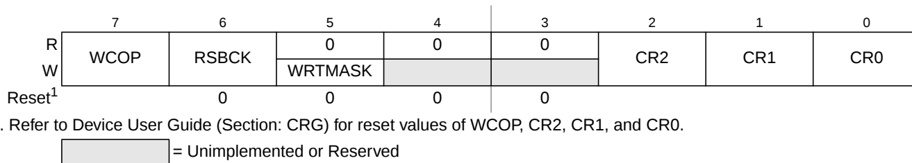
Figure 2-12. CRG COP Control Register (COPCTL)
