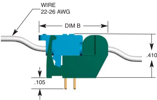
Closed Position
