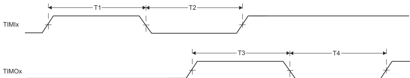
Figure 6-122. Timer Timing
