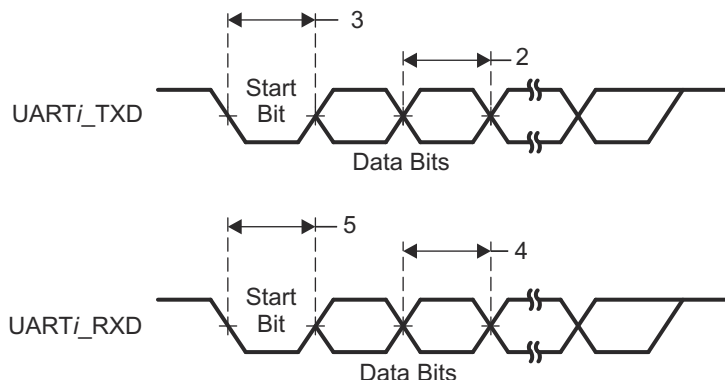
Figure 6-123. UART Timing
