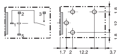
Terminal Arrangement/ Internal Connections (Bottom View)
