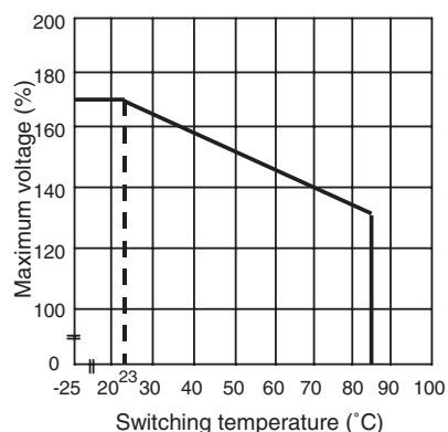
Ambient Temp. Vs Max. Voltage
