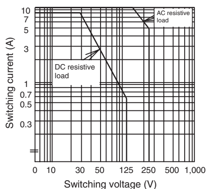
Max. Switching Power, G5LB-1
