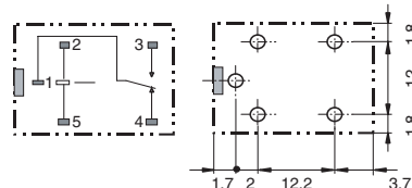
Terminal Arrangement/ Internal Connections (Bottom View)
