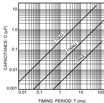
Fig. 6 One-shot time characteristics
