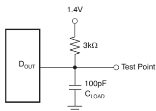
Load Circuit for t_{dO} , t_r , and t_f
