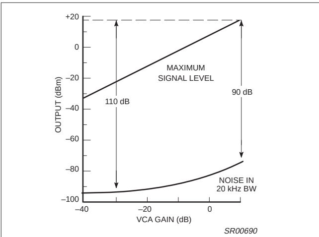
Figure 16. Dynamic range
