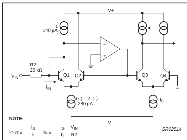
Figure 13. Simplified \Delta G Cell Schematic
