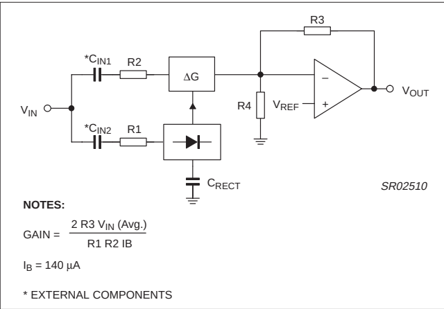
Figure 7. Basic expander
