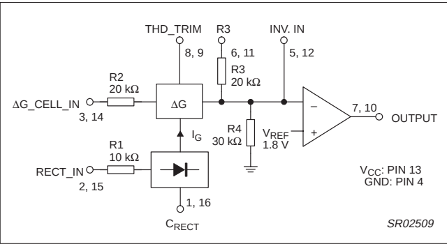
Figure 6. Chip block diagram (1 of 2 channels)
