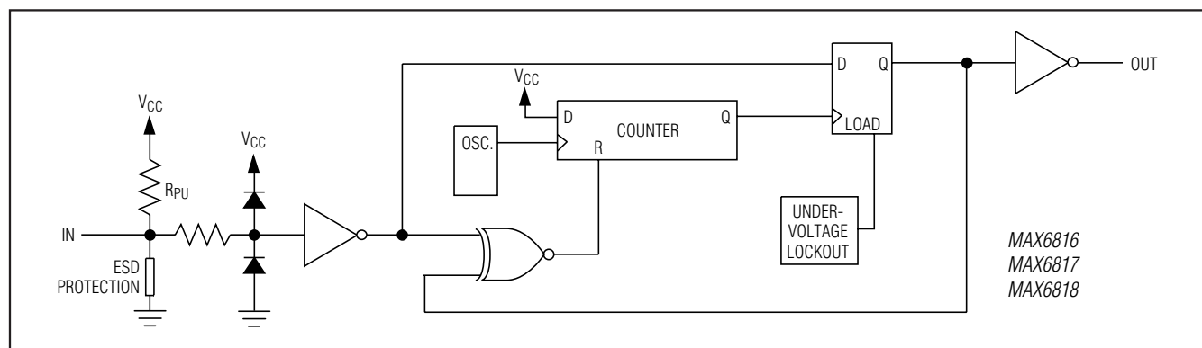
Figure 1. Block Diagram
