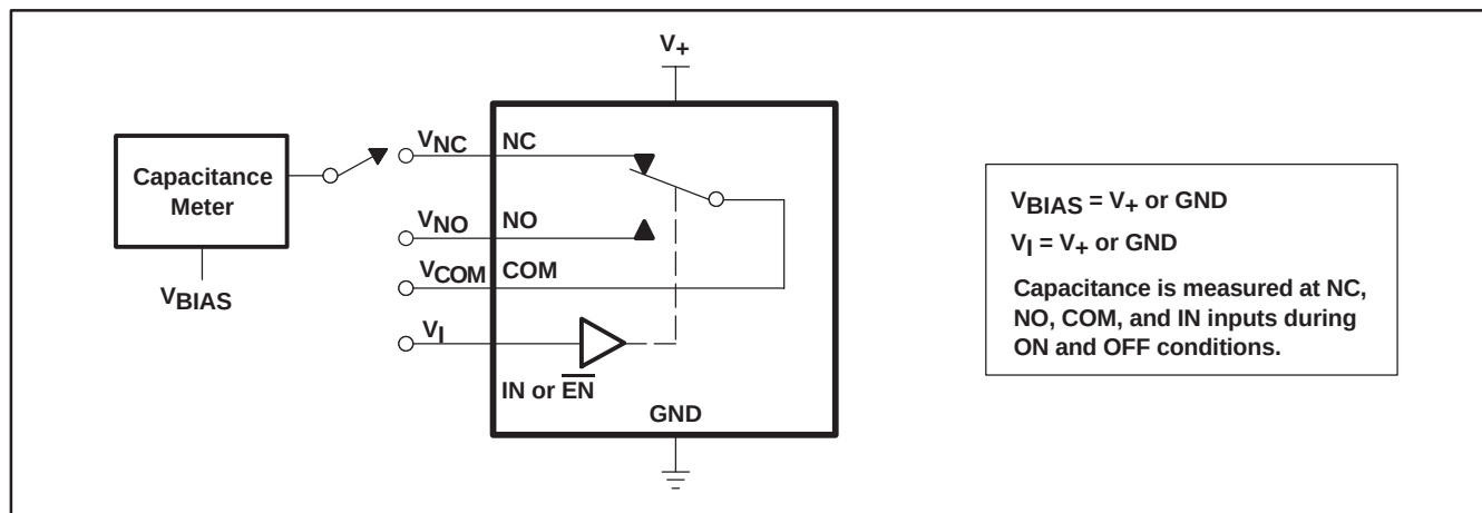
Figure 16. Capacitance ( C_I , C_{\text{COM(ON)}} , C_{\text{COM(OFF)}} , C_{\text{NC(ON)}} , C_{\text{NC(OFF)}} , C_{\text{NO(ON)}} , C_{\text{NO(OFF)}} )
