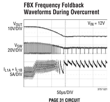
PAGE 31 CIRCUIT
