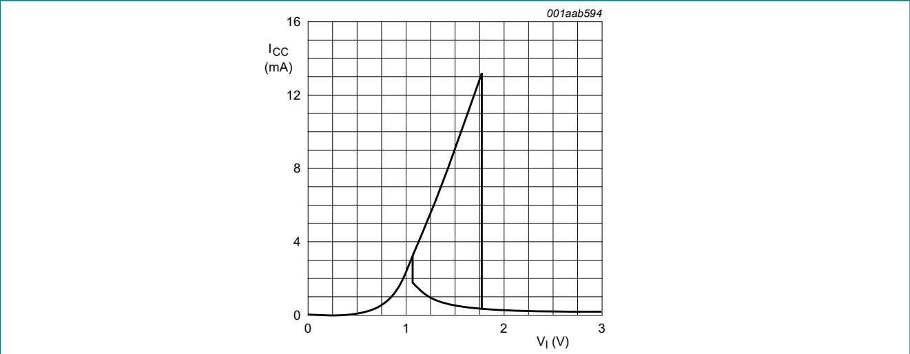
Fig. 18. Typical 74LVC1G57 transfer characteristic; V_{CC} = 3.0 V
