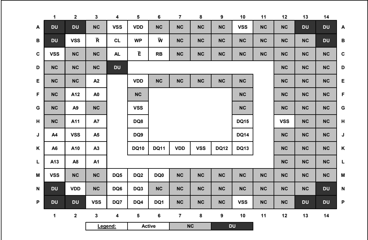
Figure 5. VFBGA153 connections (top view through package)
