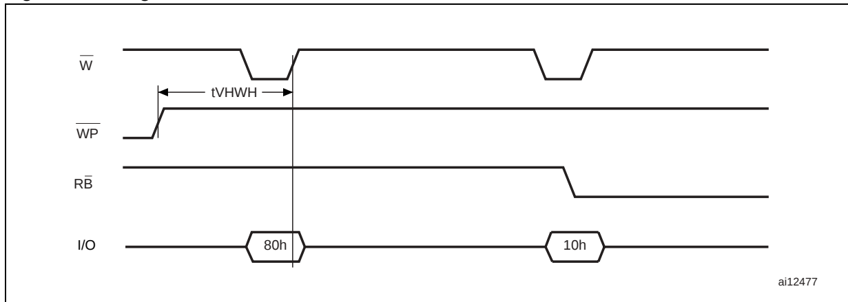
Figure 32. Program/erase enable waveforms
