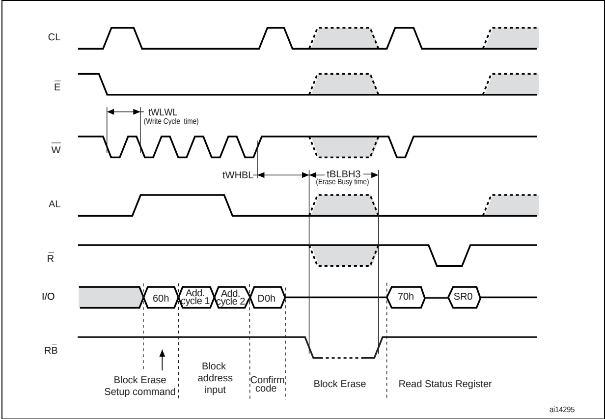
Figure 30. Block erase AC waveforms
