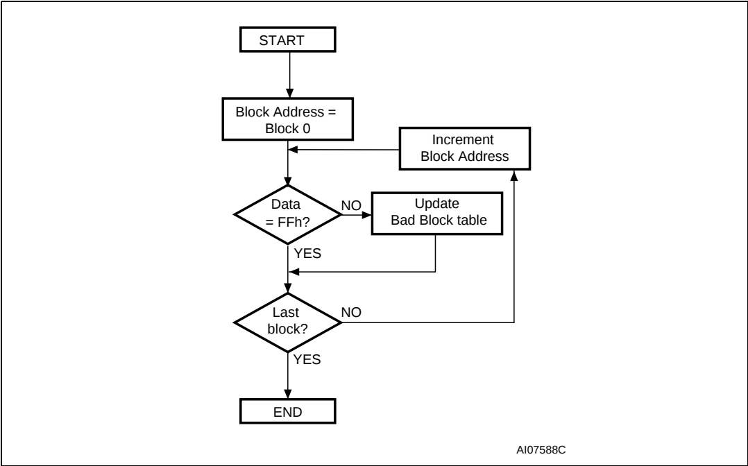
Figure 18. Bad block management flowchart
