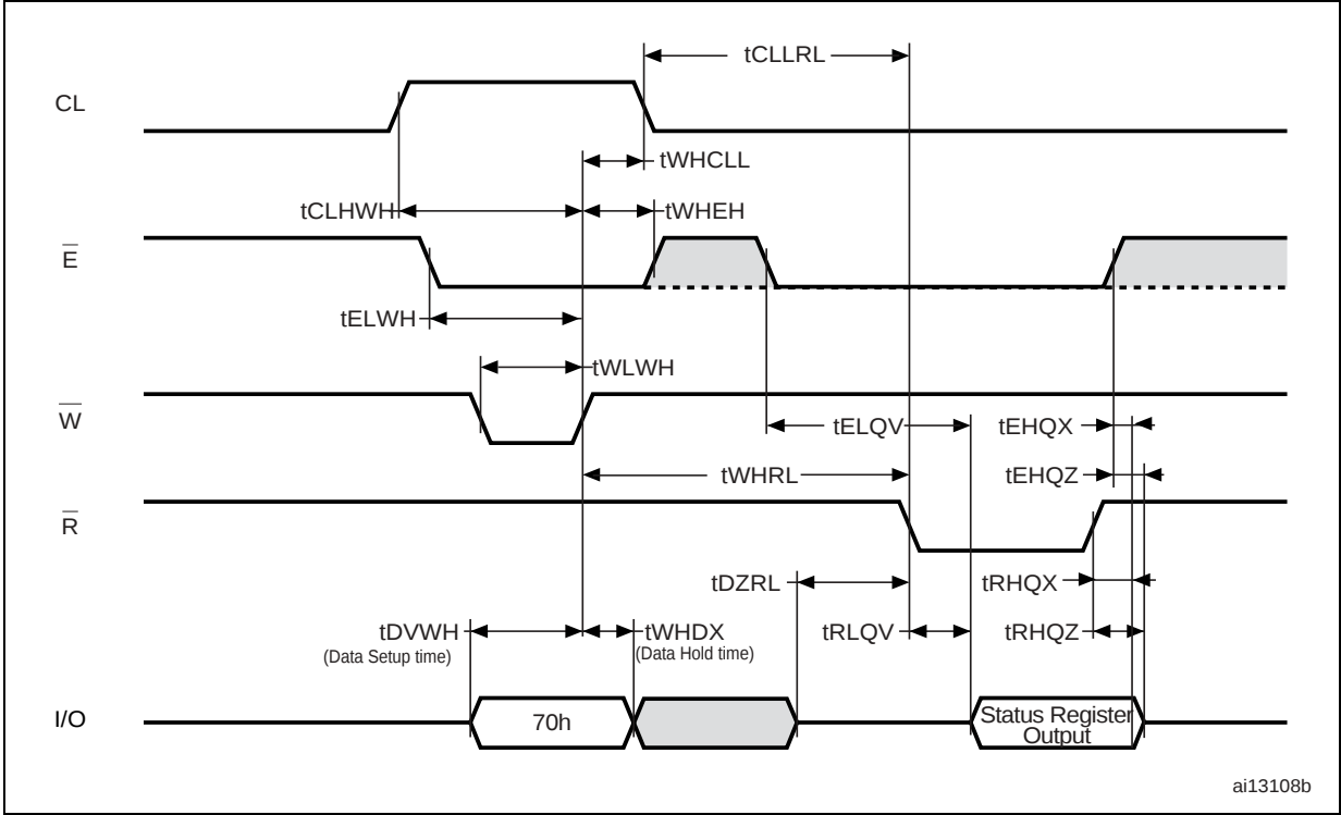
Figure 26. Read status register AC waveforms
