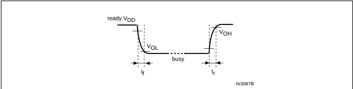
Figure 34. Ready/Busy AC waveform
