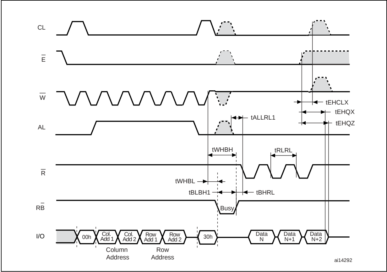
Figure 8. Read operations (intercepted by \overline{E} )
