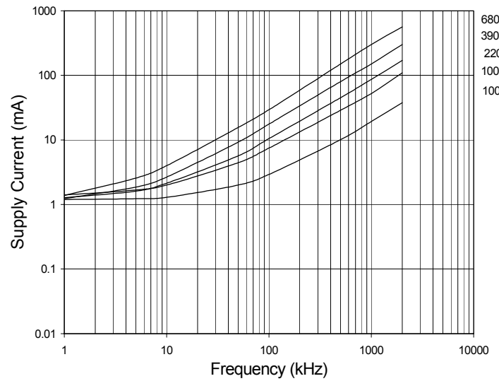
Fig. 18 Supply Current vs. Frequency V CC = 35V
