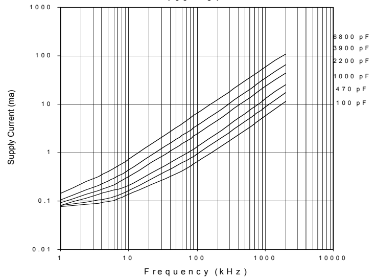
Fig. 14 Supply Current vs. Frequency V CC = 12V
