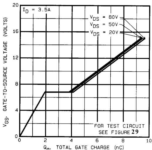
Fig 22. Typical Gate Charge Vs. Gate-to-Source Voltage
