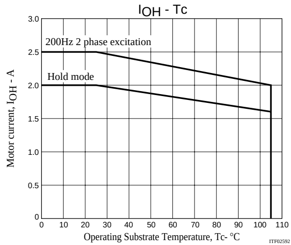
Derating Curve of Motor Current, I_{OH} , vs. STK672-430A-E Operating Substrate Temperature, T_c
