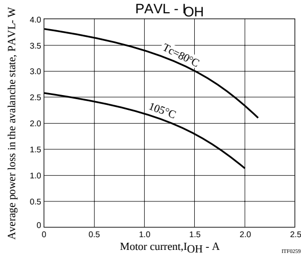
Figure 3 Allowable Loss Range, PAVL-I_{OH} During STK672-430A-E Avalanche Operations
