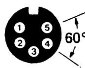
5A pole 60° contact spacing
