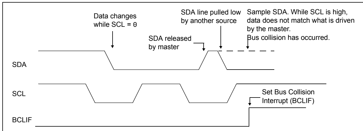
FIGURE 28-24: BUS COLLISION TIMING FOR TRANSMIT AND ACKNOWLEDGE
