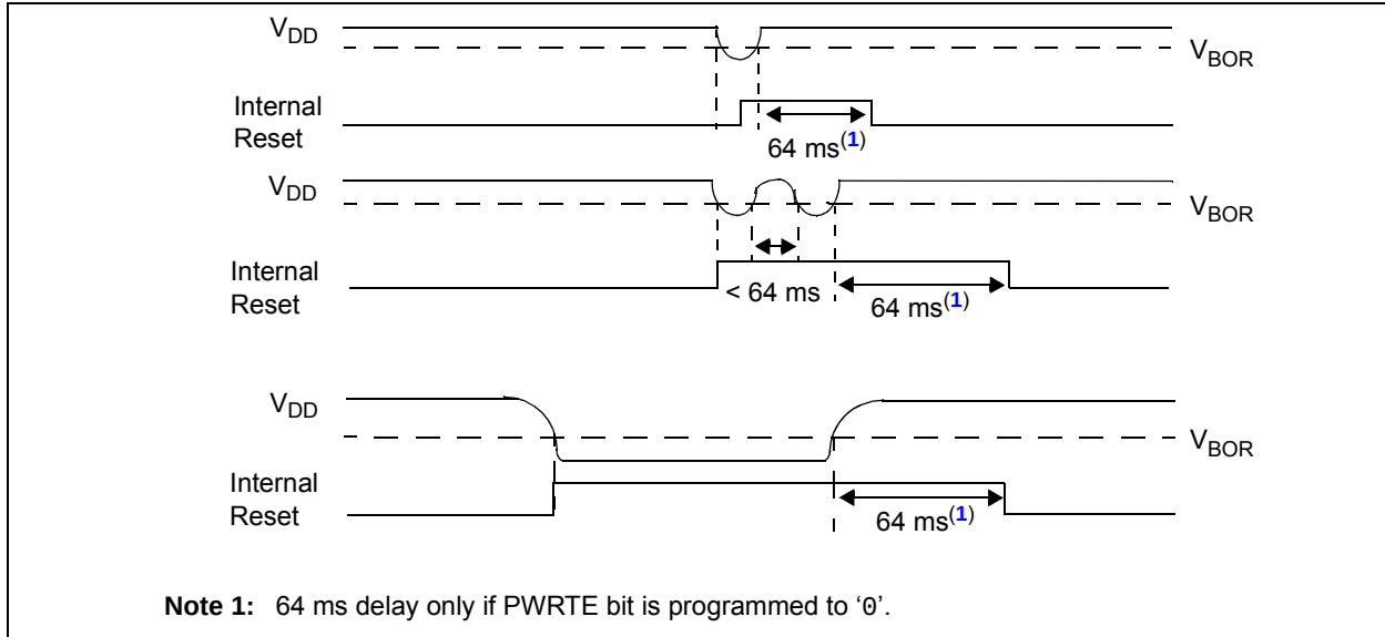
FIGURE 13-3: BROWN-OUT SITUATIONS
