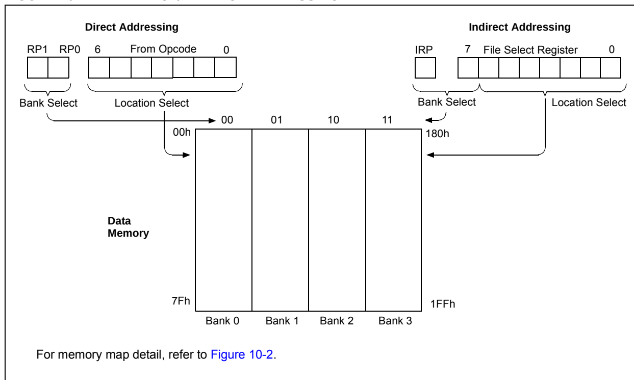
FIGURE 10-4: DIRECT/INDIRECT ADDRESSING
