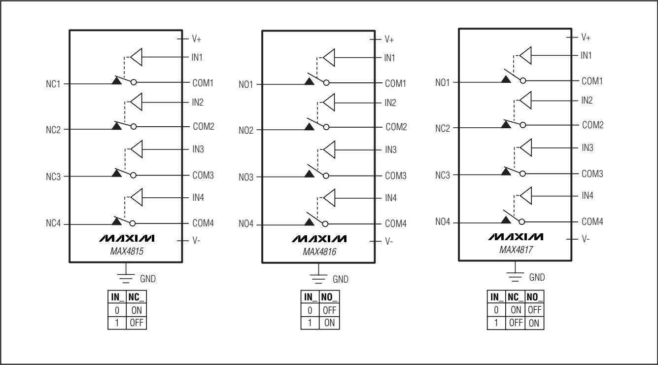
Functional Diagram
