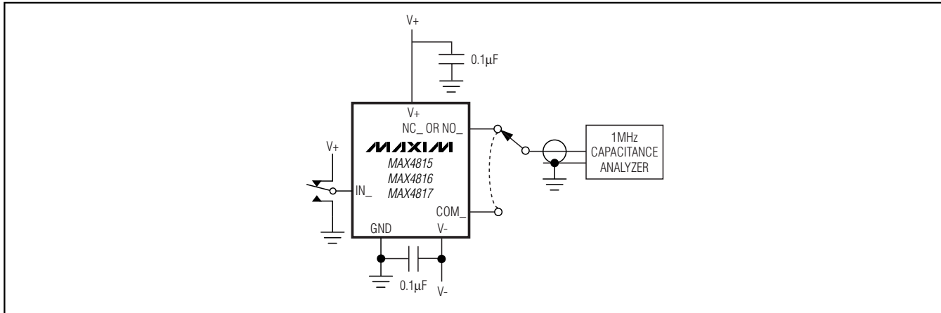
Figure 5. Channel Off-/On-Capacitance
