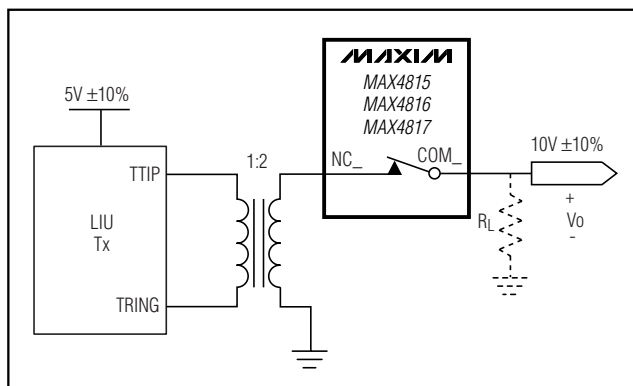
Figure 1. Fault Protection
