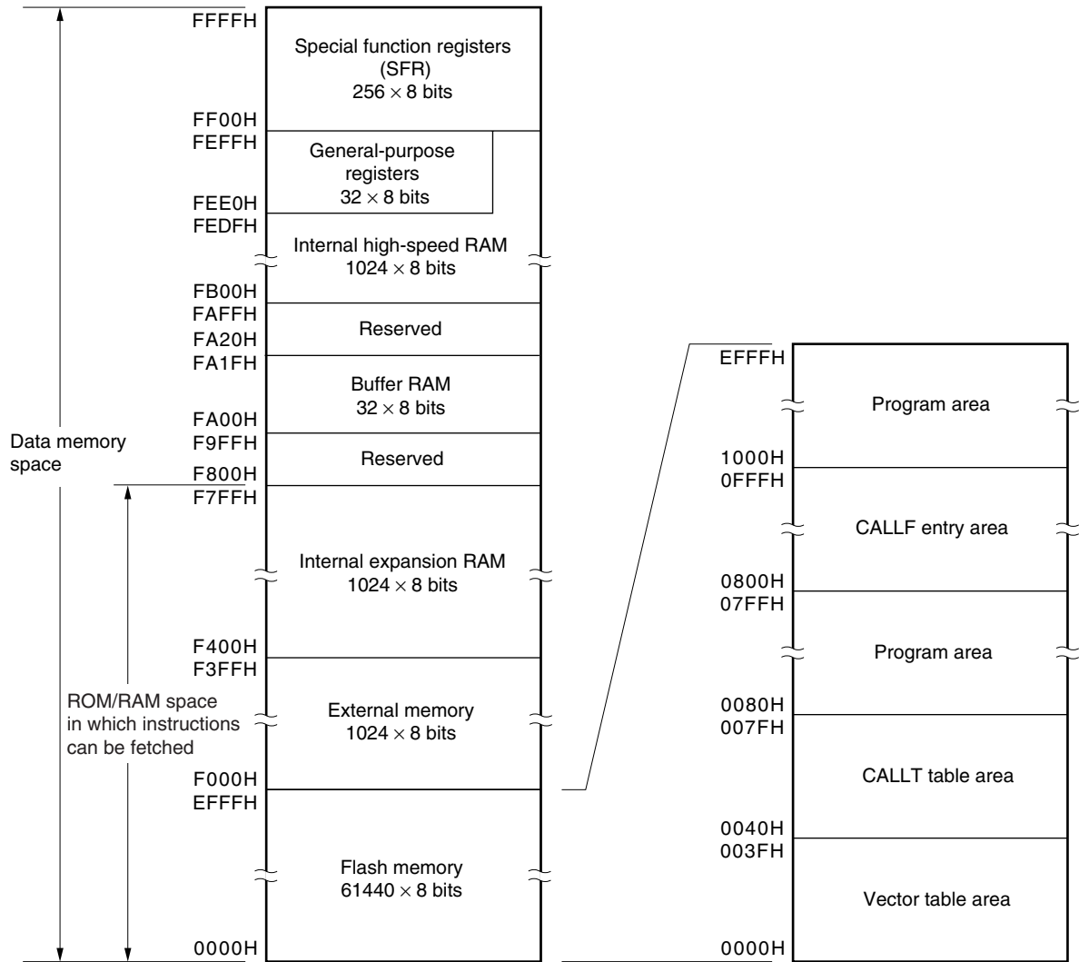
Figure 3-5. Memory Map ( \mu PD78F0148)
