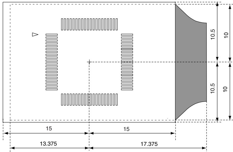
Figure B-6. Restricted Area on Target System (80-Pin GK Package)
