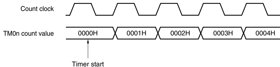
Figure 7-40. Start Timing of 16-Bit Timer Counter 0n (TM0n)
