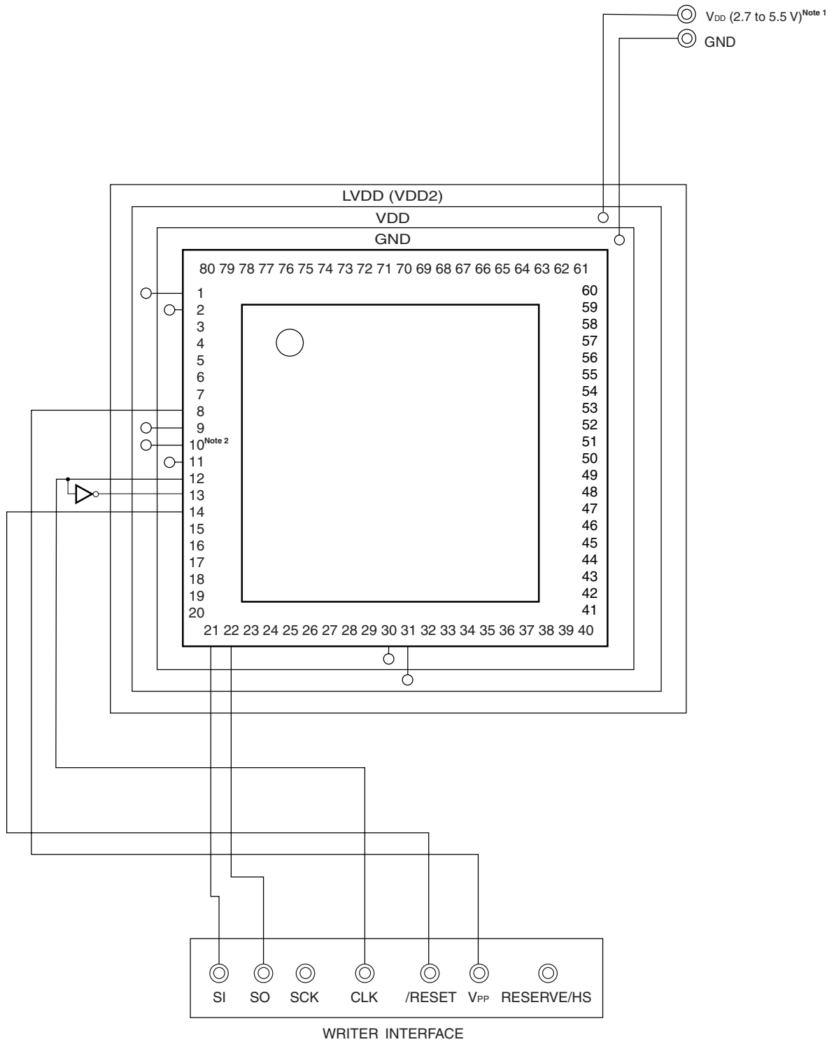
Figure 28-7. Example of Wiring Adapter for Flash Memory Writing in UART (UART6) Mode
