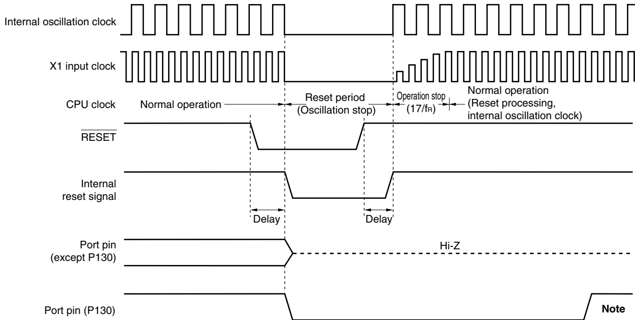
Figure 22-2. Timing of Reset by \overline{\text{RESET}} Input
