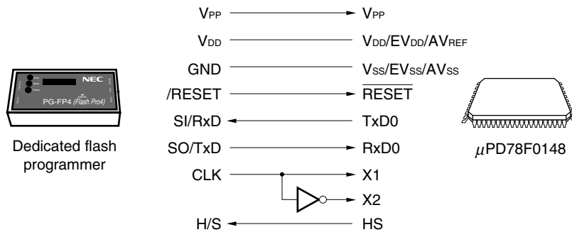
Figure 28-12. Communication with Dedicated Flash Programmer (UART0 + HS)
