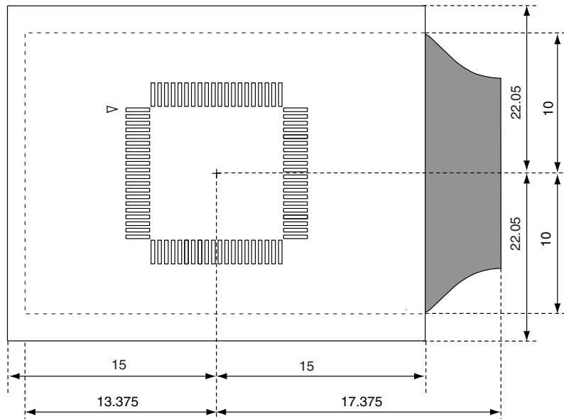
Figure B-7. Restricted Area on Target System (80-Pin GC Package)
