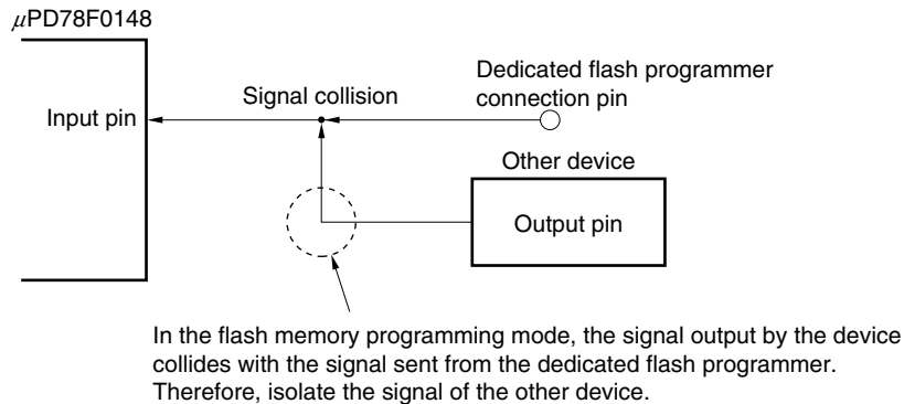
Figure 28-15. Signal Collision (Input Pin of Serial Interface)
