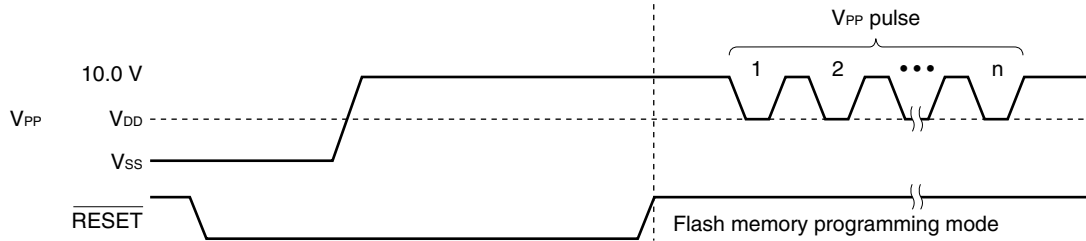
Figure 28-19. Flash Memory Programming Mode
