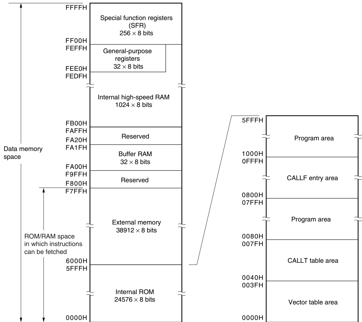
Figure 3-1. Memory Map ( \mu PD780143)
