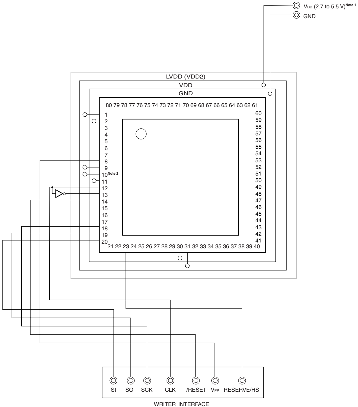
Figure 28-4. Example of Wiring Adapter for Flash Memory Writing in 3-Wire Serial I/O (CSI10 + HS) Mode
