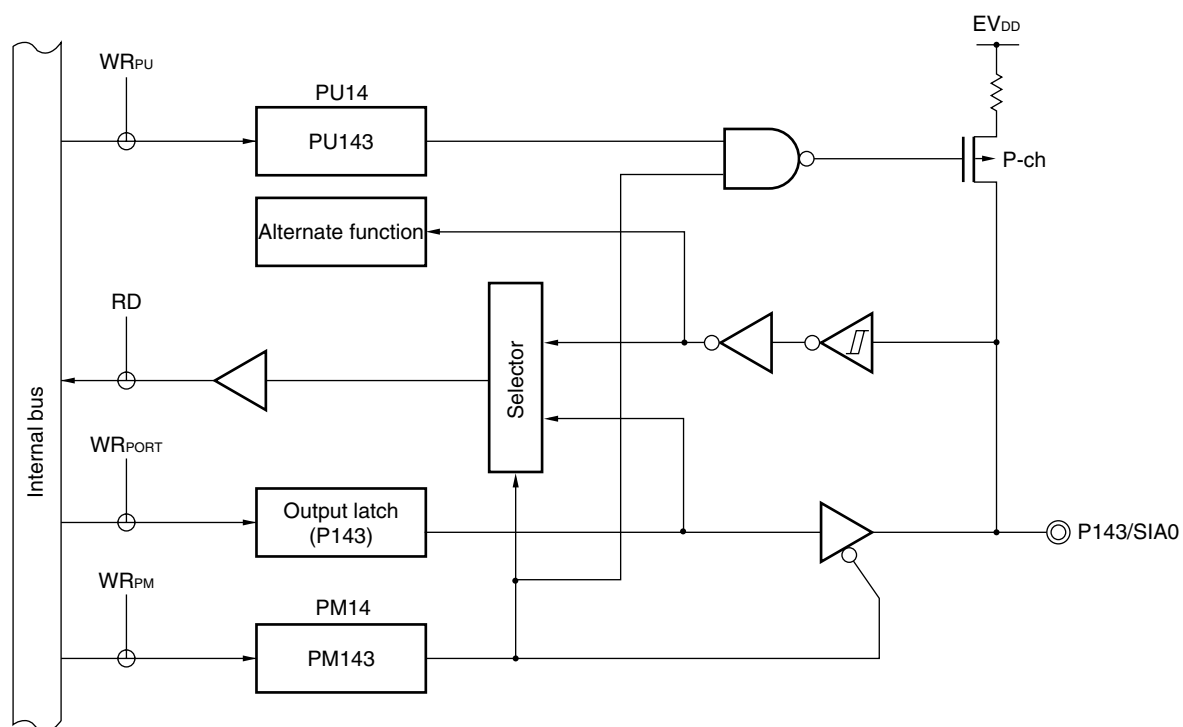
Figure 4-24. Block Diagram of P143
