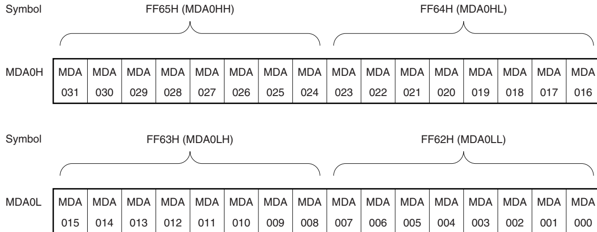
Figure 18-3. Format of Multiplication/Division Data Register A0 (MDA0H, MDA0L)
