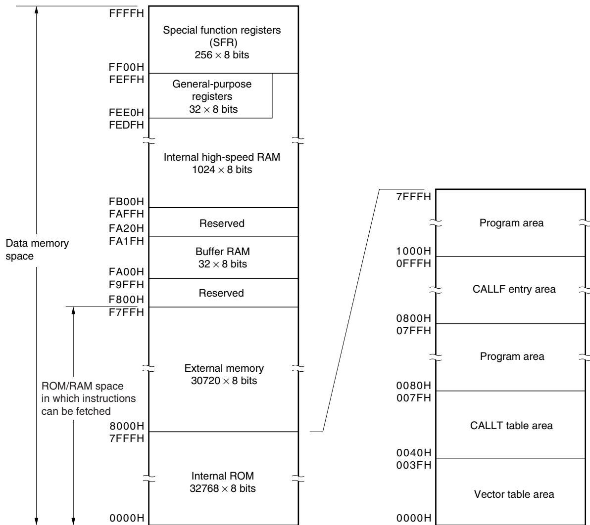
Figure 3-2. Memory Map ( \mu PD780144)
