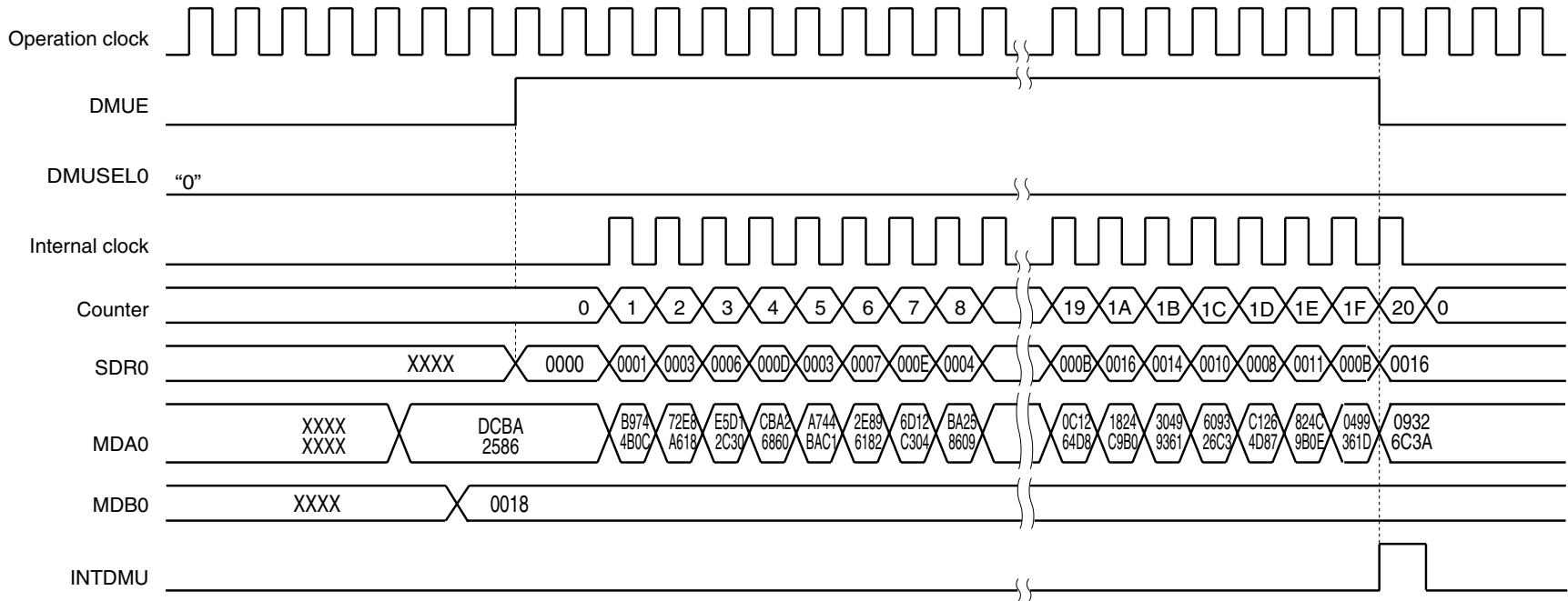
Figure 18-7. Timing Chart of Division Operation (DCBA2586H ÷ 0018H)
