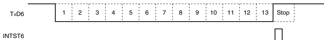
Figure 15-23. SBF Transmission
