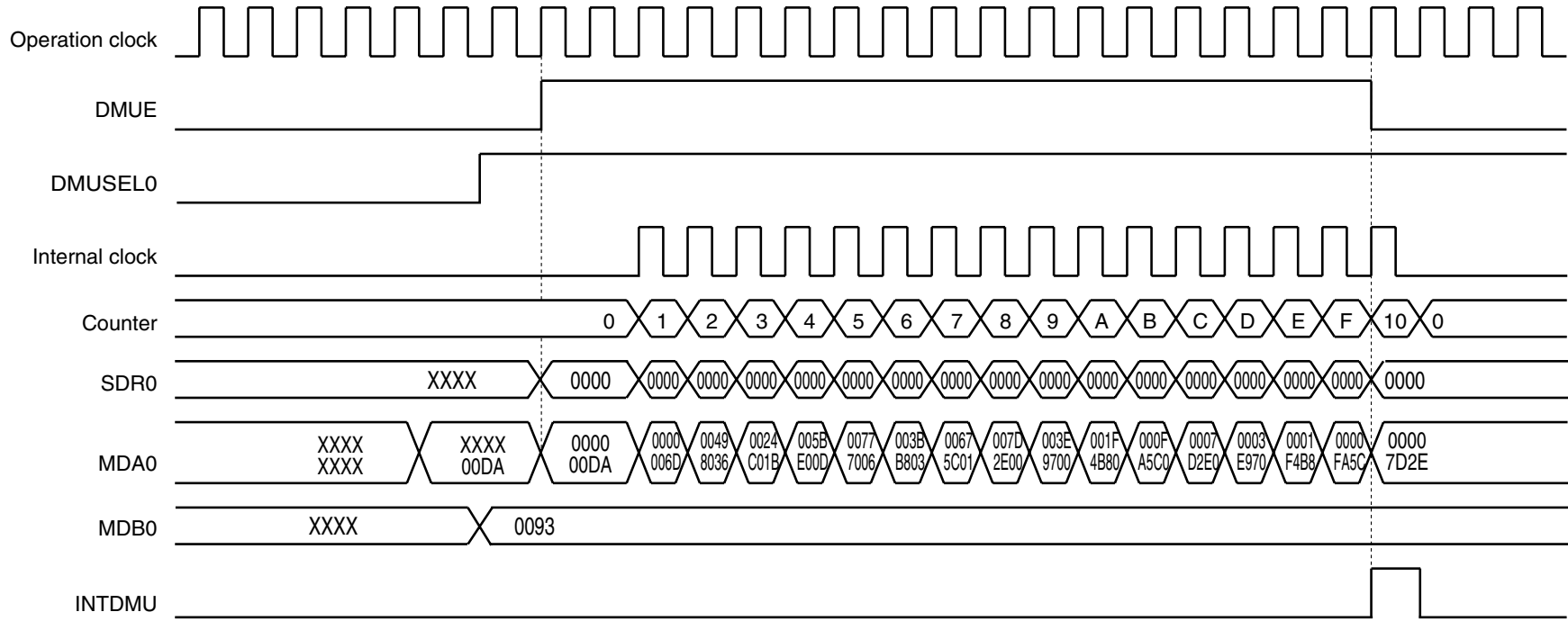
Figure 18-6. Timing Chart of Multiplication Operation (00DAH × 0093H)
