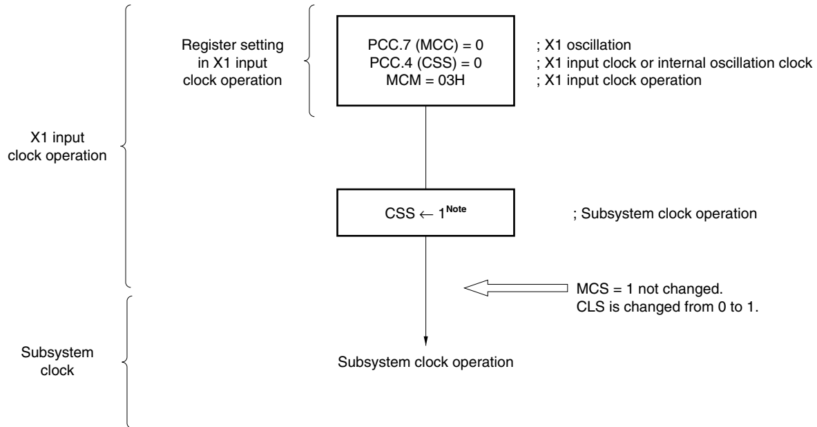
Figure 6-16. Switching from X1 Input Clock to Subsystem Clock (Flowchart)
