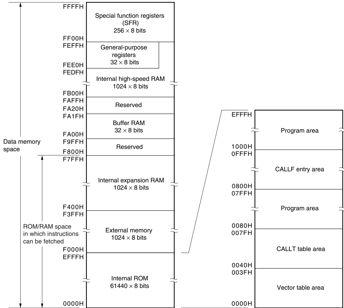
Figure 3-4. Memory Map ( \mu PD780148)
