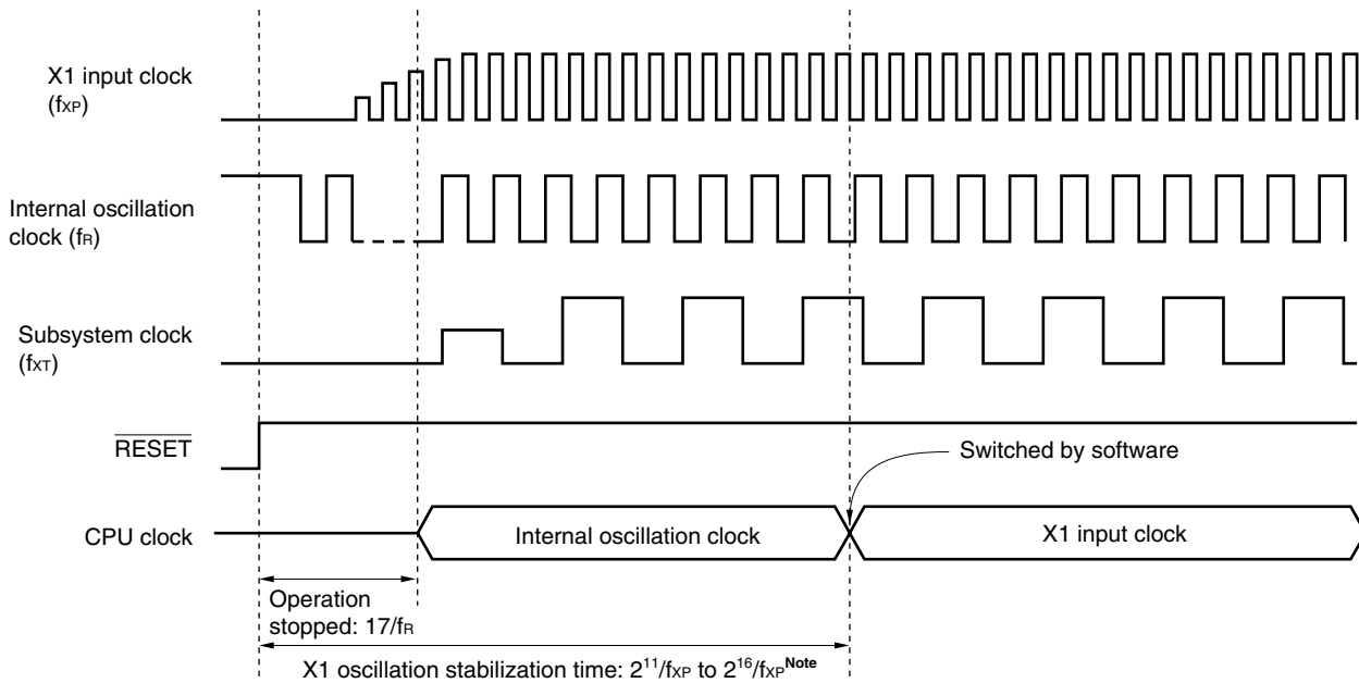
Figure 6-12. Timing Diagram of CPU Default Start Using Internal Oscillator
