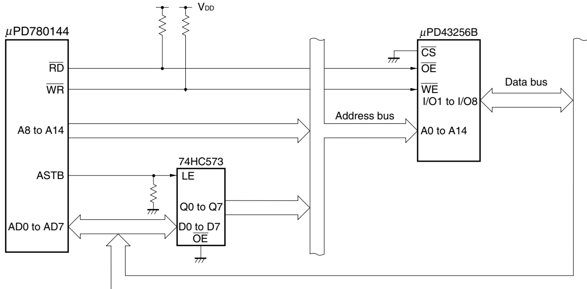
Figure 5-9. Connection Example of \mu PD780144 and Memory
