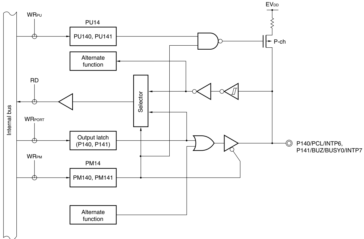
Figure 4-22. Block Diagram of P140 and P141
