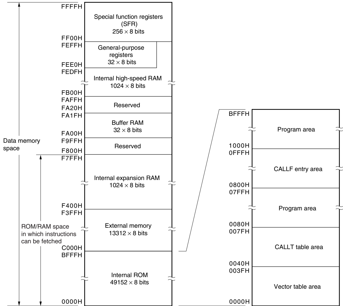
Figure 3-3. Memory Map ( \mu PD780146)
