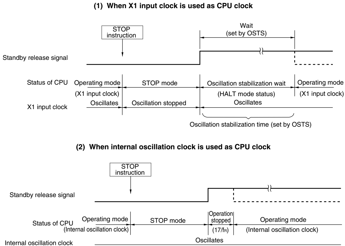
Figure 21-6. STOP Mode Release by Interrupt Request Generation
