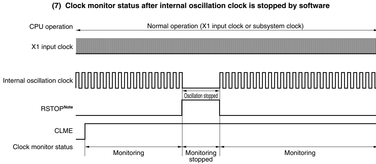
Figure 23-3. Timing of Clock Monitor (4/4)
