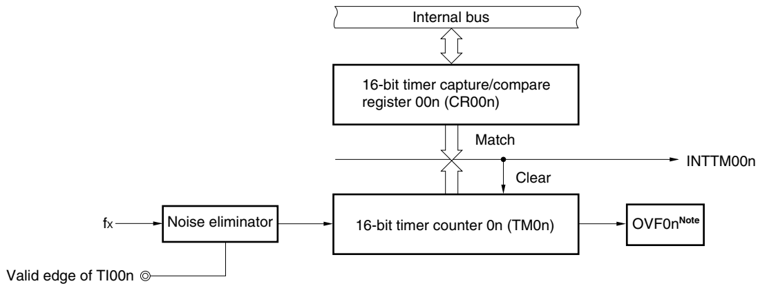
Figure 7-32. Configuration Diagram of External Event Counter
