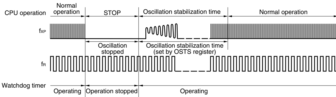
Figure 11-5. Operation in STOP Mode (CPU Clock: X1 Input Clock, WDT Operation Clock: Internal Oscillation Clock)
