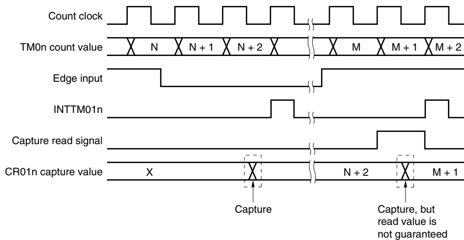
Figure 7-42. Capture Register Data Retention Timing
