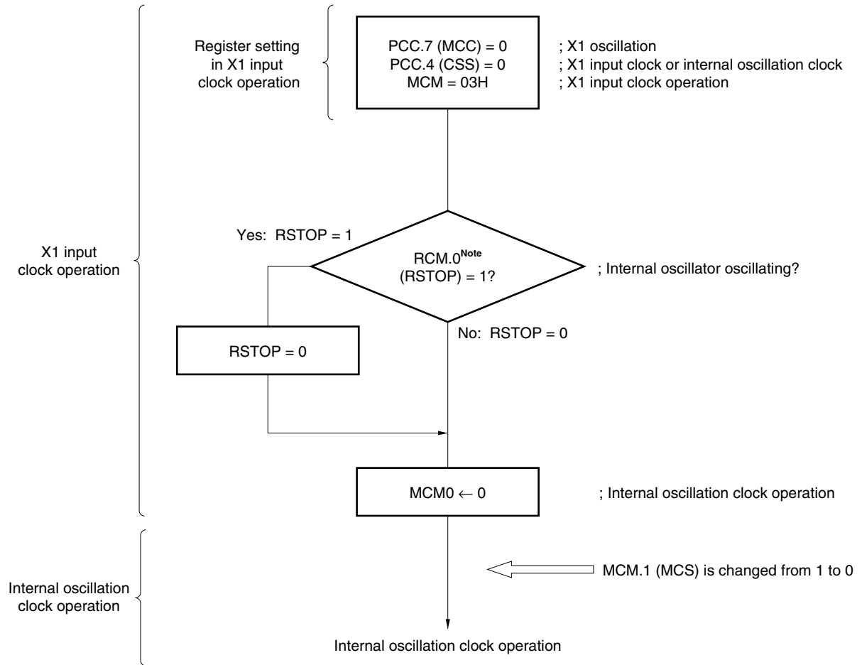
Figure 6-15. Switching from X1 Input Clock to Internal Oscillation Clock (Flowchart)
