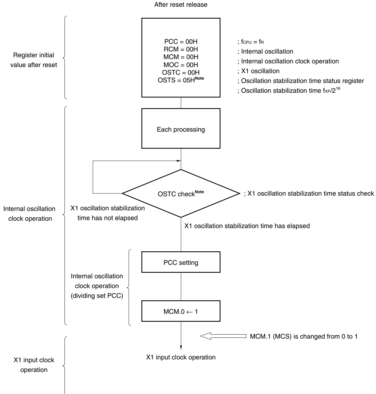
Figure 6-14. Switching from Internal Oscillation Clock to X1 Input Clock (Flowchart)
