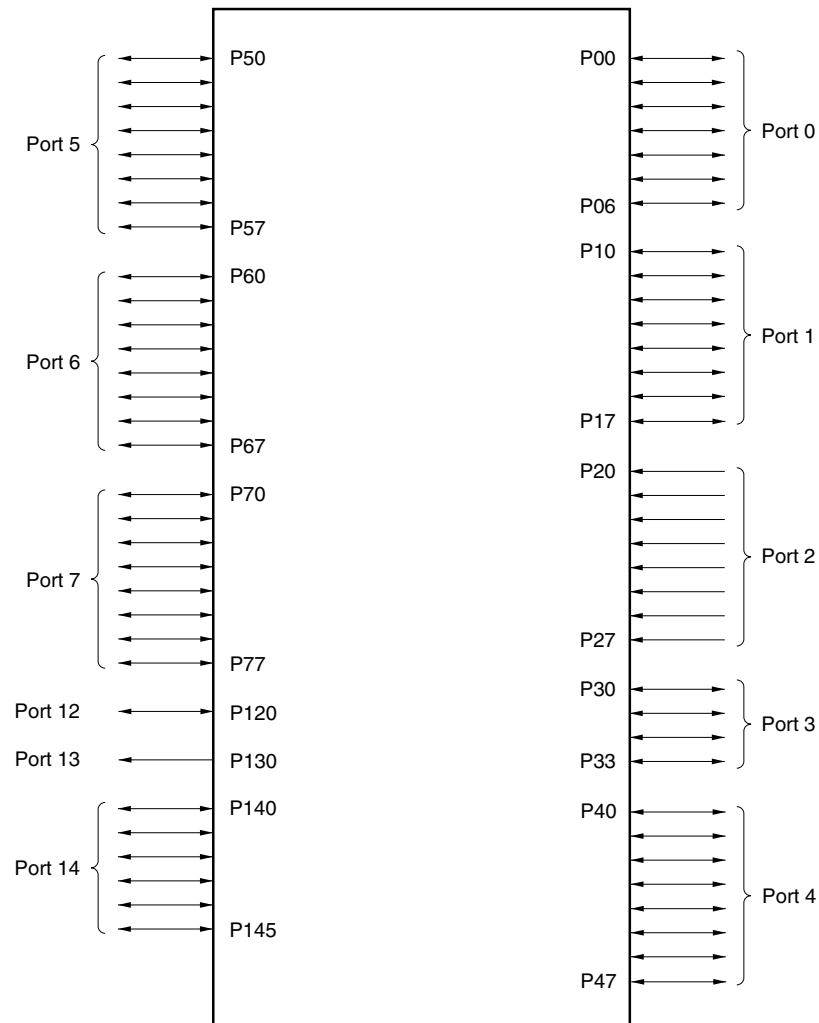
Figure 4-1. Port Types
