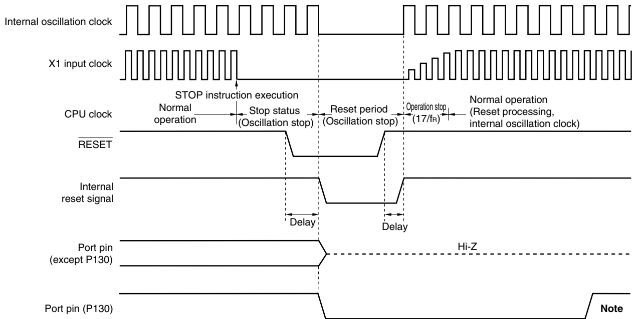
Figure 22-4. Timing of Reset in STOP Mode by \overline{\text{RESET}} Input
