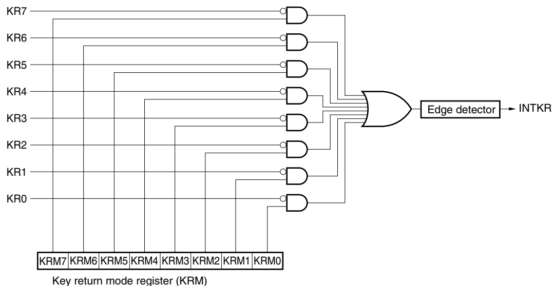
Figure 20-1. Block Diagram of Key Interrupt
