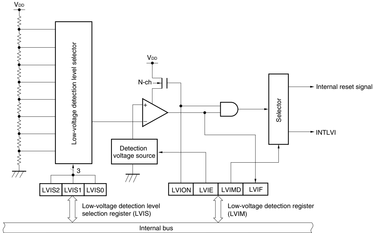
Figure 25-1. Block Diagram of Low-Voltage Detector
