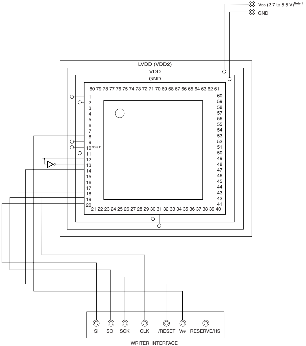
Figure 28-3. Example of Wiring Adapter for Flash Memory Writing in 3-Wire Serial I/O (CSI10) Mode
