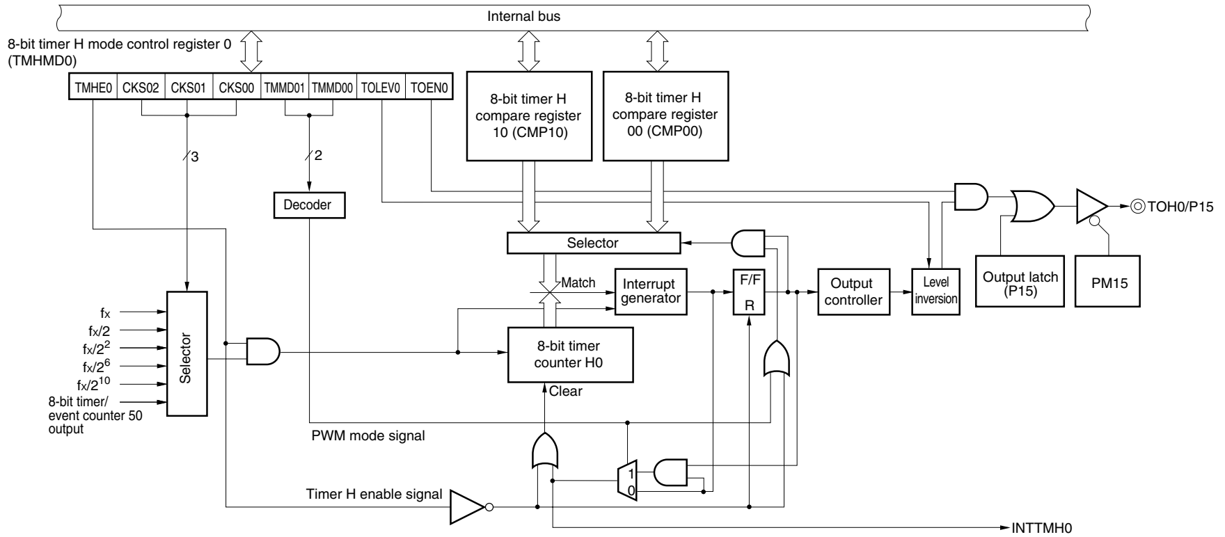
Figure 9-1. Block Diagram of 8-Bit Timer H0
