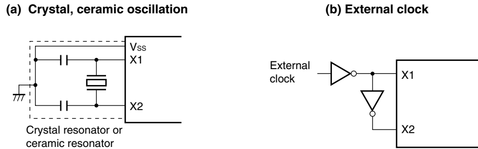
Figure 6-8. Examples of External Circuit of X1 Oscillator
