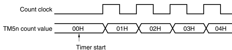
Figure 8-16. 8-Bit Timer Counter 5n Start Timing
