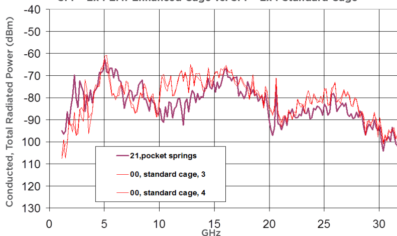
SFP+ 2x4 EMI-Enhanced Cage vs. SFP+ 2x4 Standard Cage
