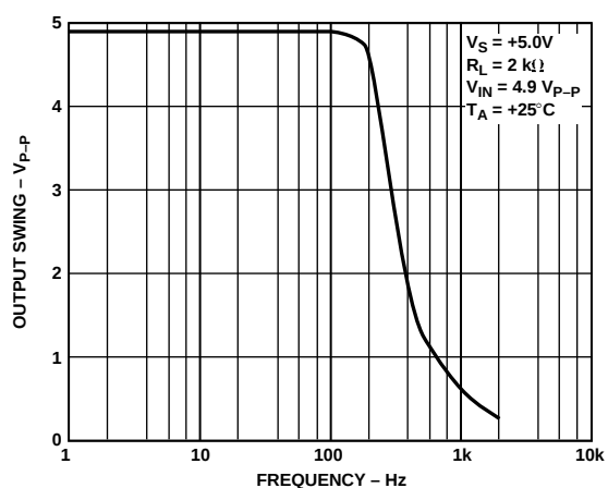
Figure 12. Closed-Loop Output Voltage Swing vs. Frequency
