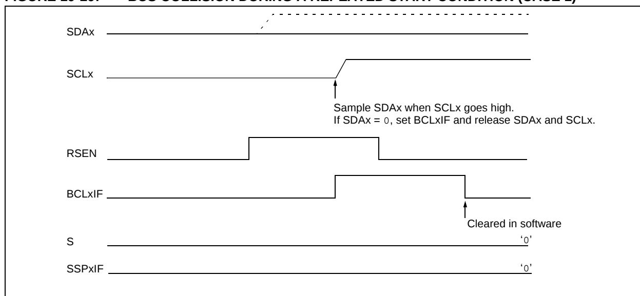
FIGURE 19-29: BUS COLLISION DURING A REPEATED START CONDITION (CASE 1)
