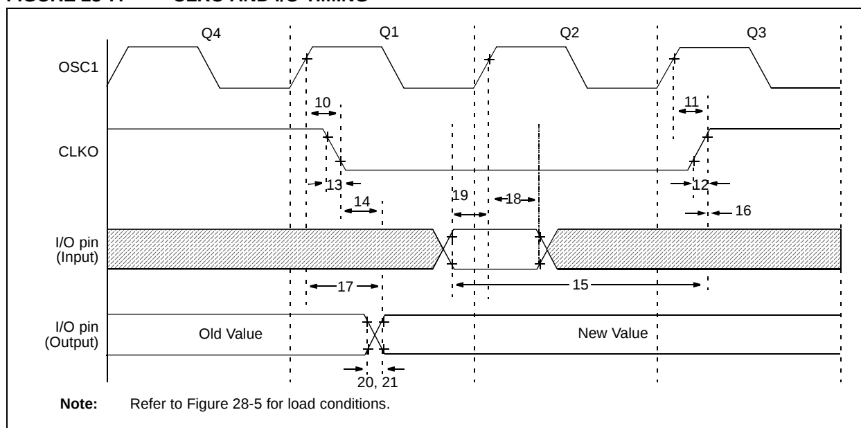
FIGURE 28-7: CLKO AND I/O TIMING
