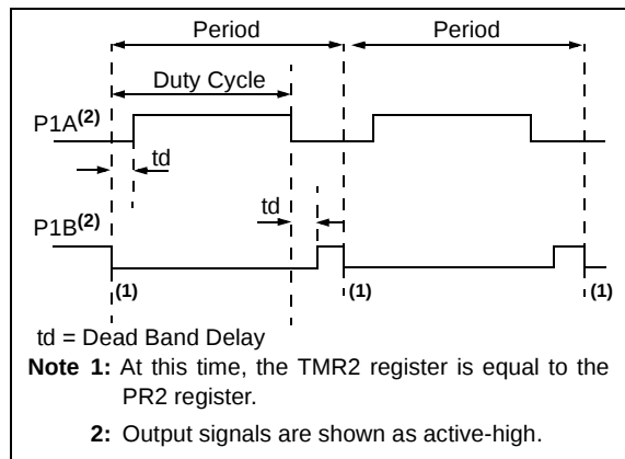
FIGURE 18-4: HALF-BRIDGE PWM OUTPUT
