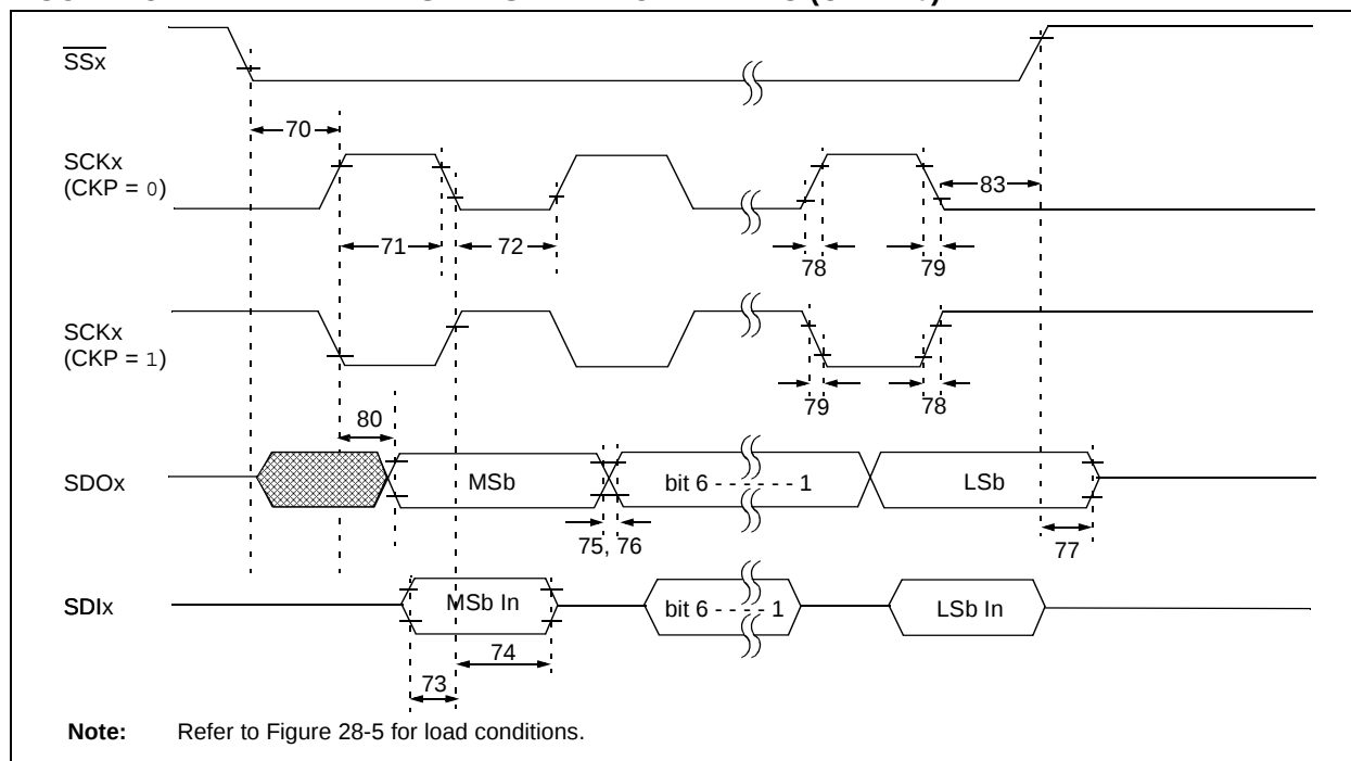
FIGURE 28-17: EXAMPLE SPI™ SLAVE MODE TIMING (CKE = 0)
