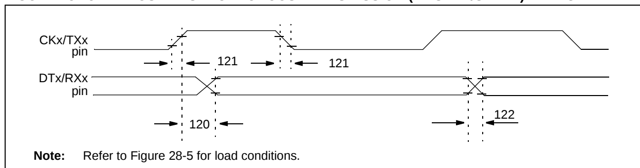
FIGURE 28-23: EUSART SYNCHRONOUS TRANSMISSION (MASTER/SLAVE) TIMING
