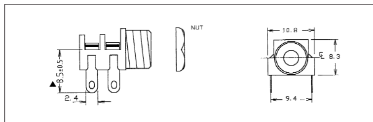
S6/BB mono switched 3.5mm Jack Socket. Panel mounting with solder tags. Also available with Special 'C' Contact to suit Far Eastern plugs.
