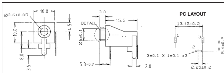
JYO-36A mono switched 3.5mm Jack Socket. Stand-off right angle PCB mounting with threadless nose.
