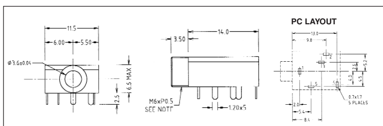
JYS-35 stereo switched 3.5mm Jack Socket. Right angle PCB mounting. Supplied with ring nut.
