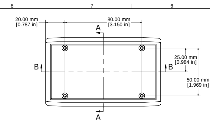
ASSEMBLY - TOP
